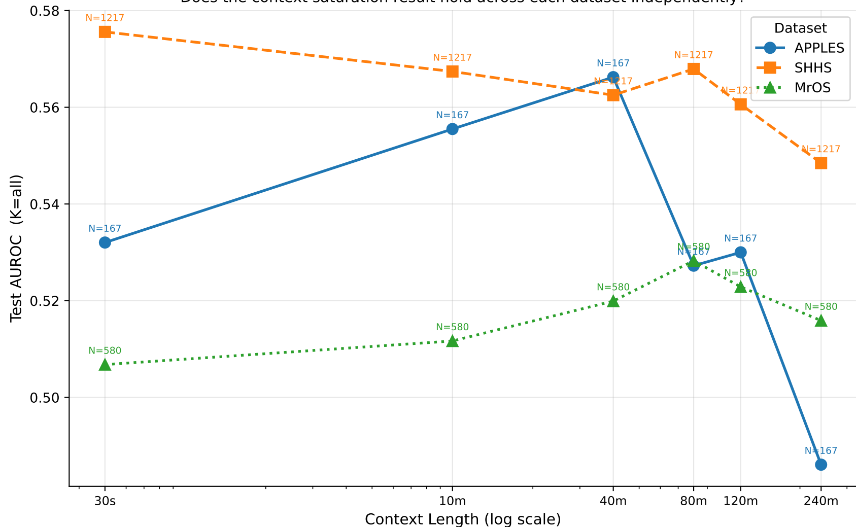
Cohort-Stratified Saturation — sleepiness_binary (LSTM) Does the context saturation result hold across each dataset independently?
