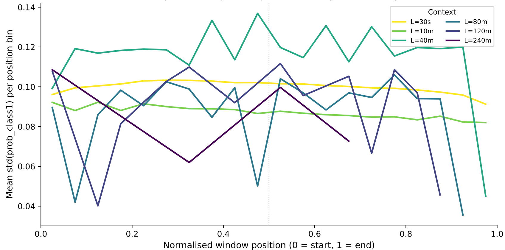
Prediction Variance vs Night Position — sleepiness_binary (LSTM) Lower variance = position-independent predictions (longer context may flatten this)
