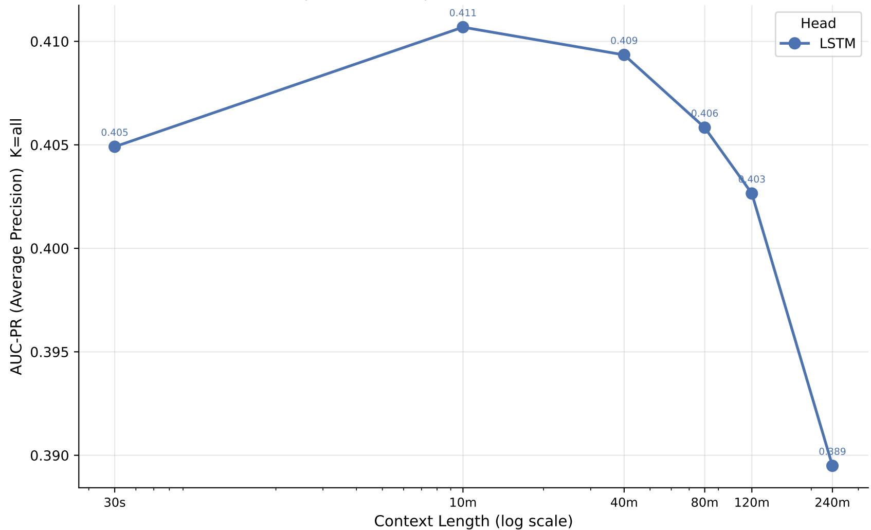
AUC-PR vs Context Length — sleepiness_binary Does precision-recall performance saturate like AUROC?
