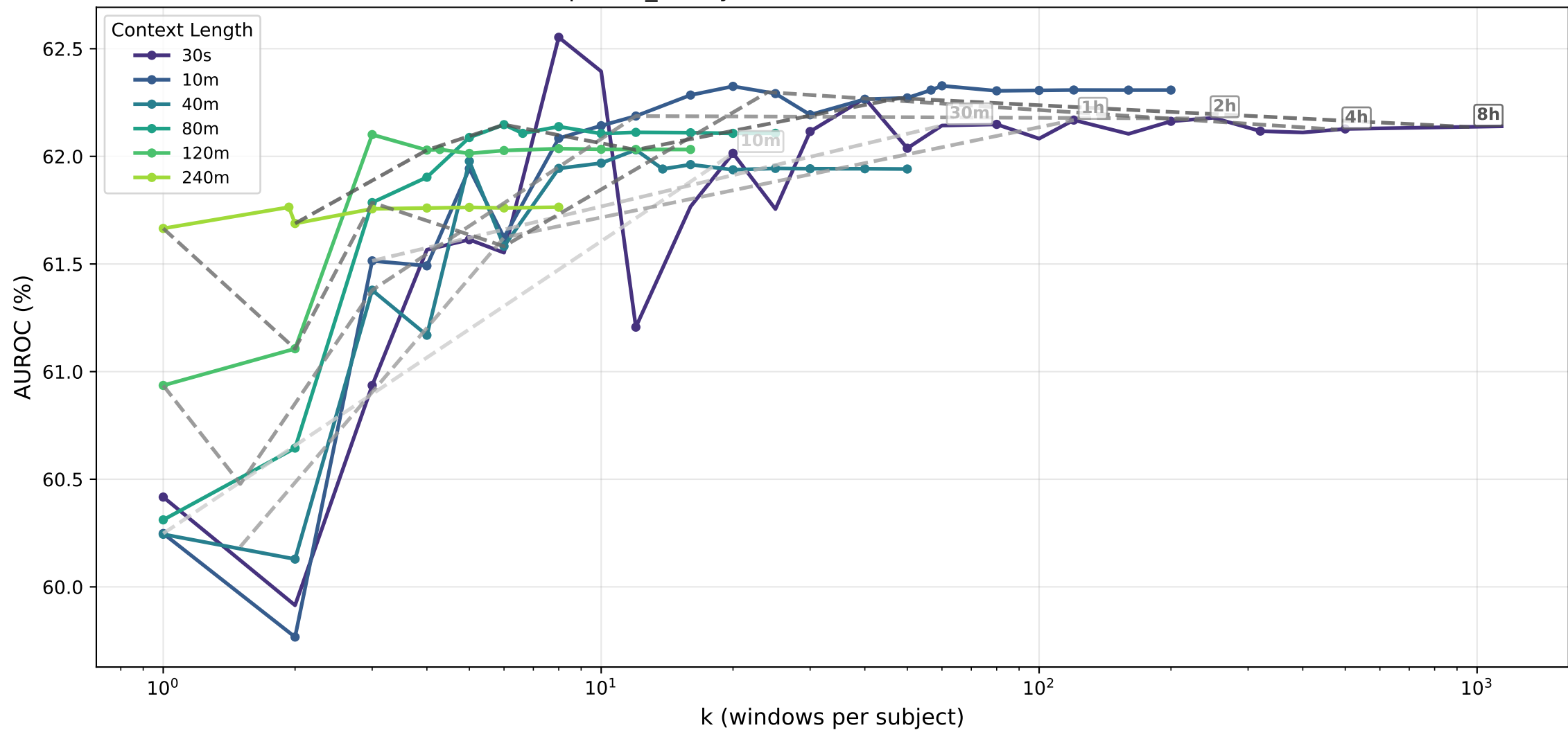
sleepiness_binary · transformer — AUROC (%) vs k
