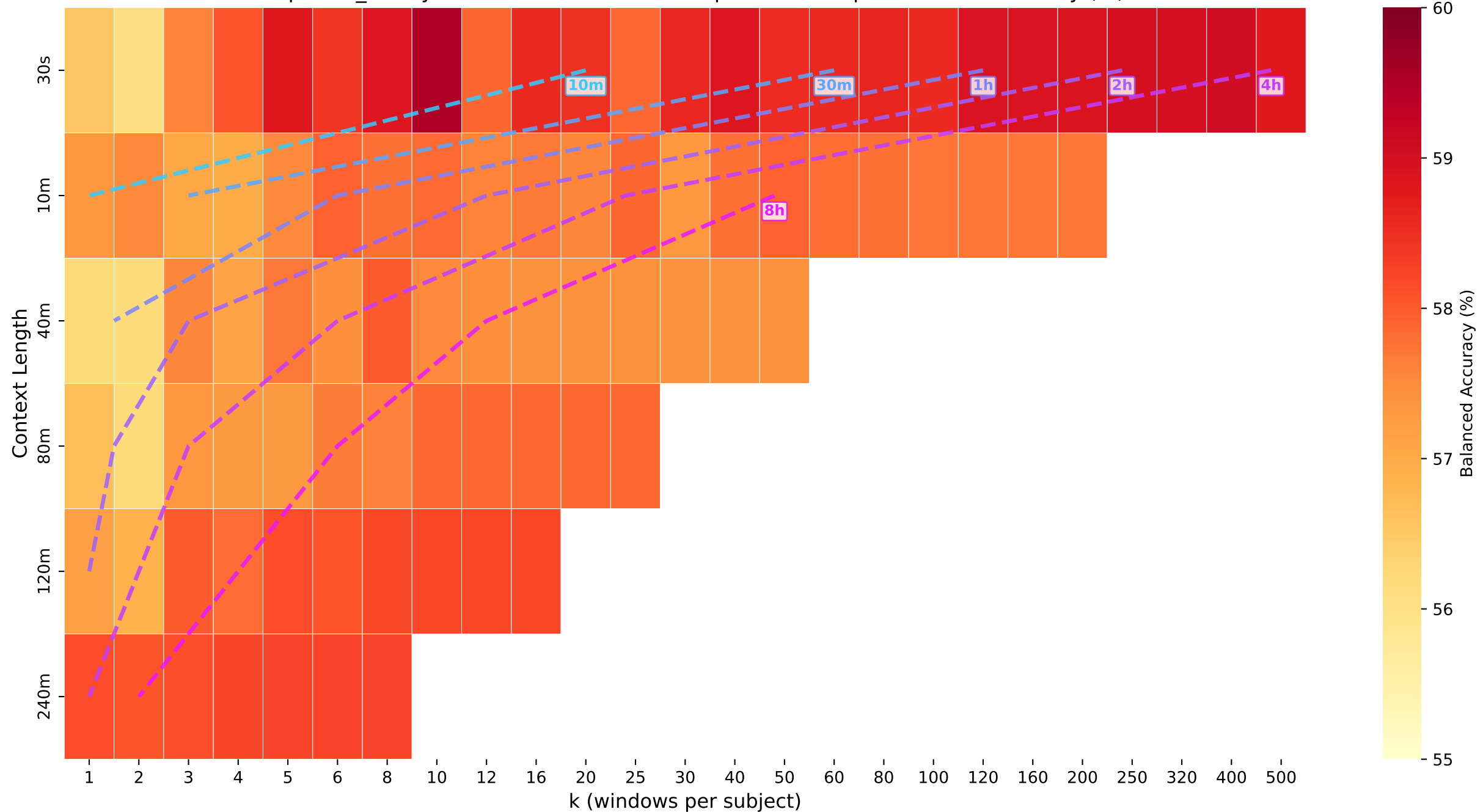
sleepiness_binary · transformer — Iso-Compute Heatmap: Balanced Accuracy (%)
