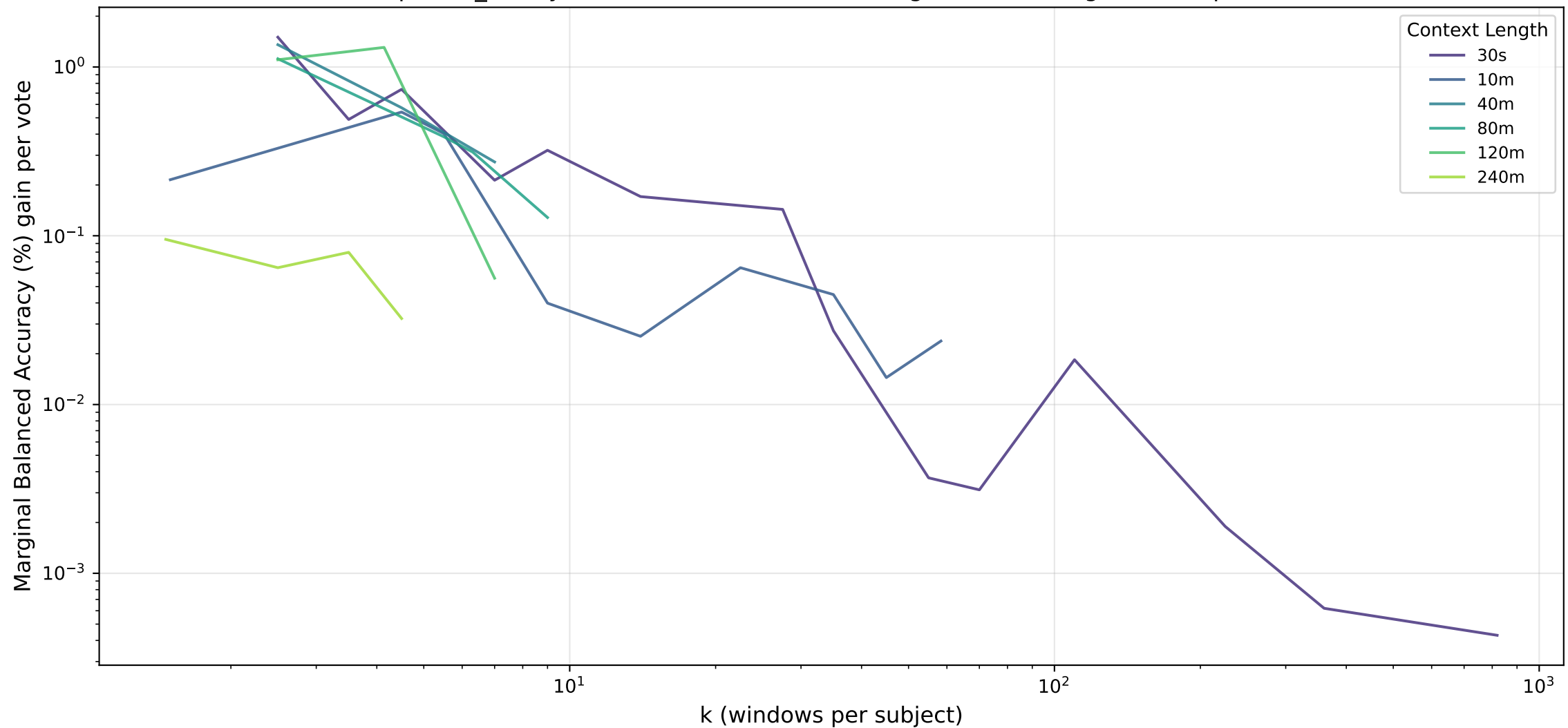
sleepiness_binary · transformer — Diminishing Returns: Marginal Gain per Vote
