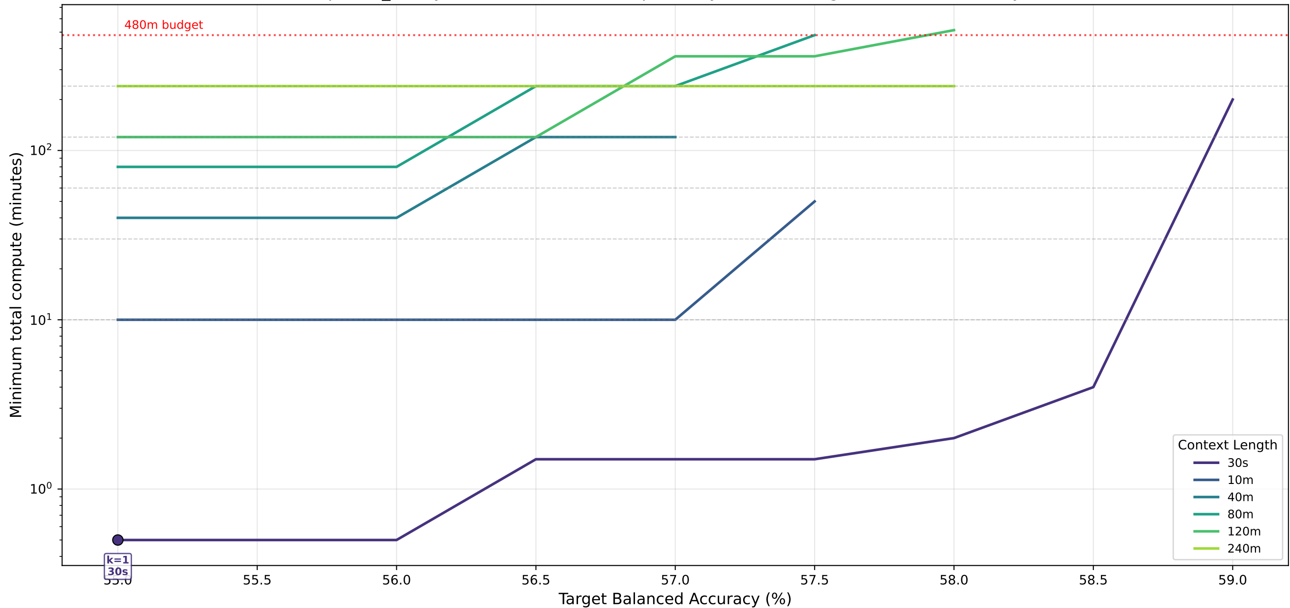
sleepiness_binary · transformer — Cheapest Way to Reach Target Balanced Accuracy (%)
