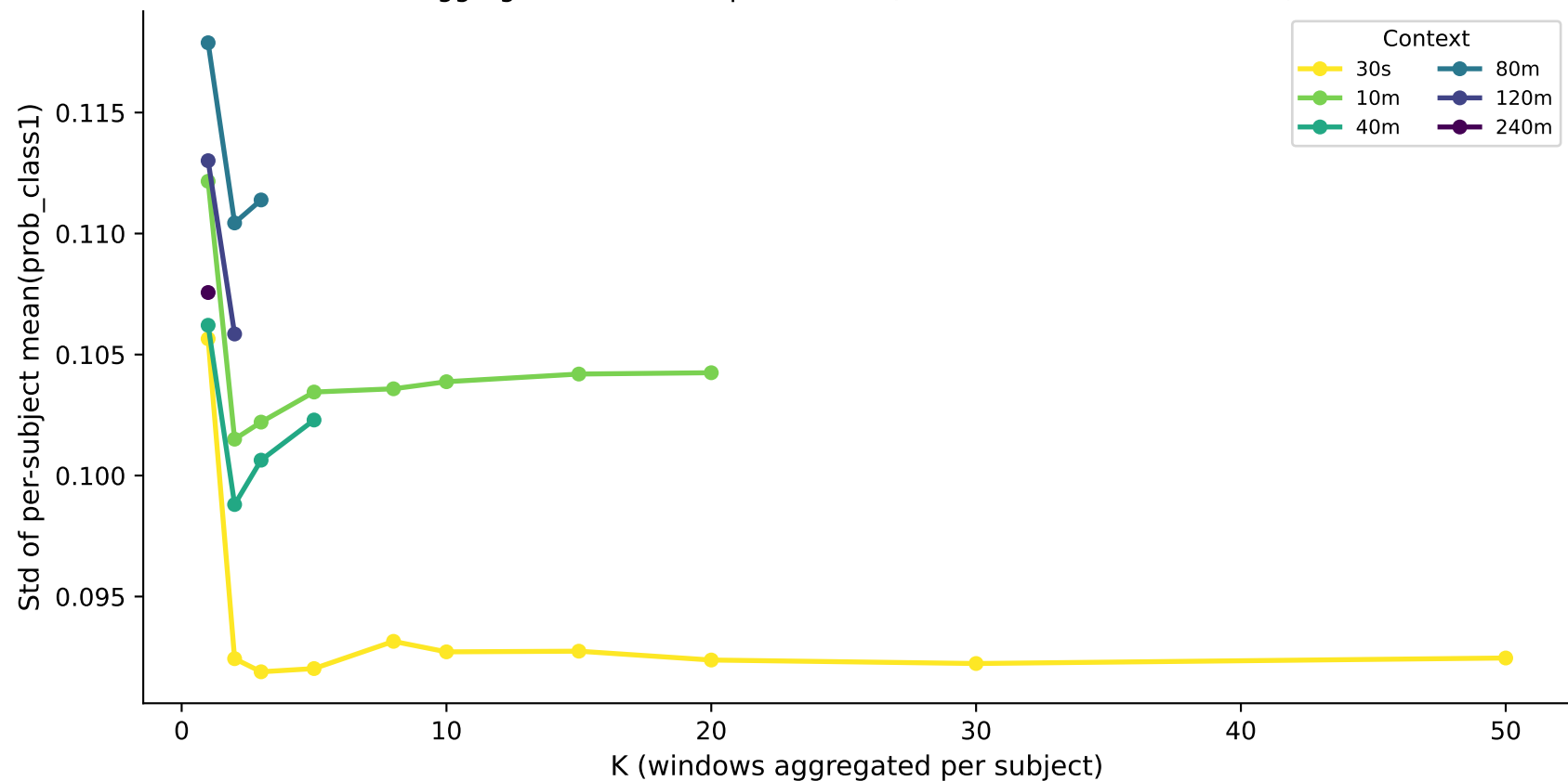
Prediction Variance vs K — sleepiness_binary (TRANSFORMER) Aggregation stabilises predictions (lower std = more consistent)
