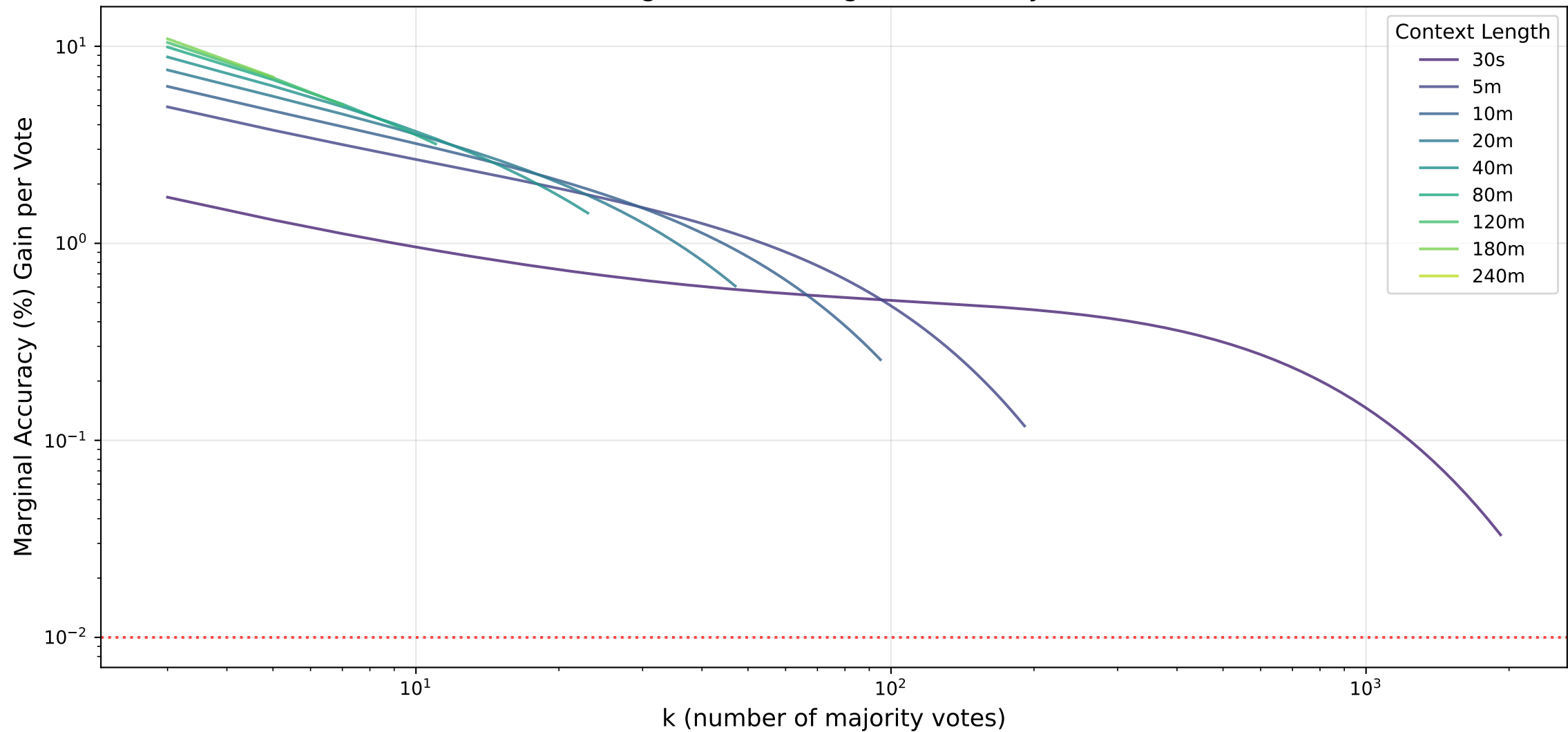
Diminishing Returns: Marginal Accuracy (%) Gain
