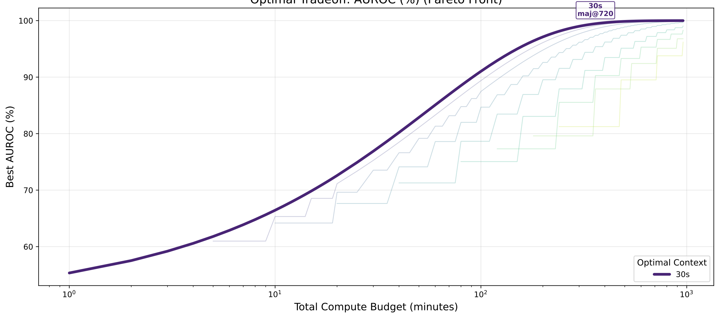
Optimal Tradeoff: AUROC (%) (Pareto Front)
