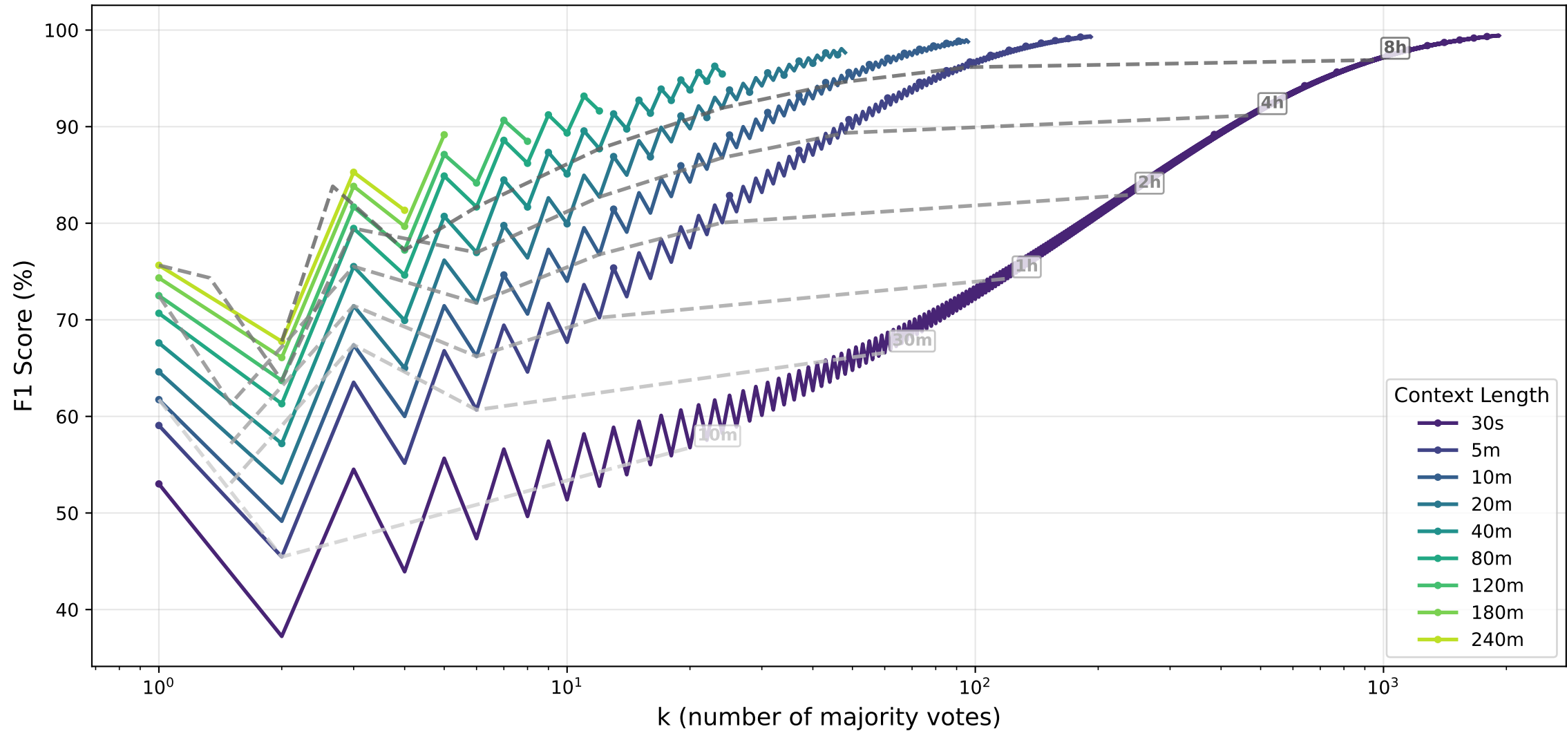
F1 Score (%) vs k by Context Length
