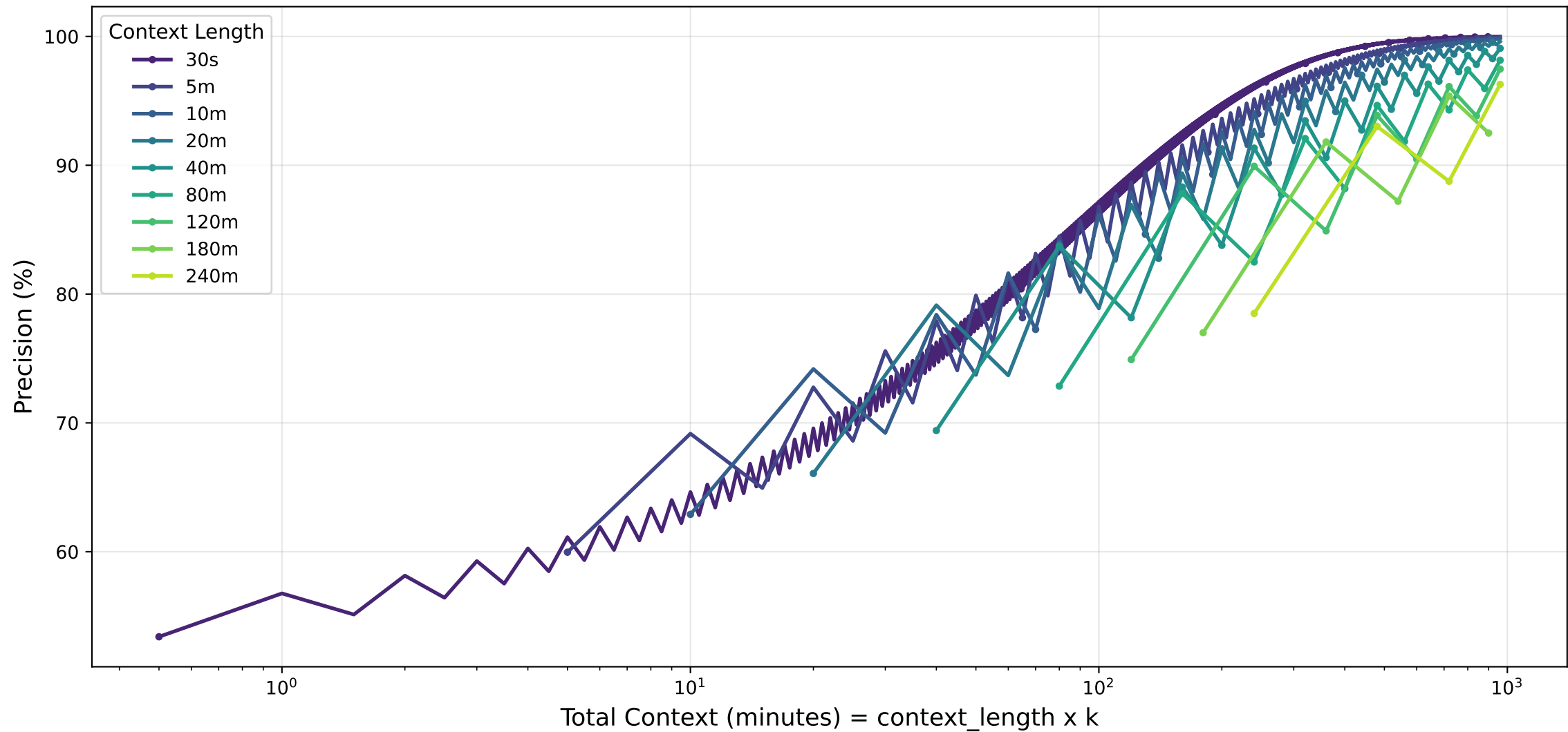
Precision (%) vs Total Context
