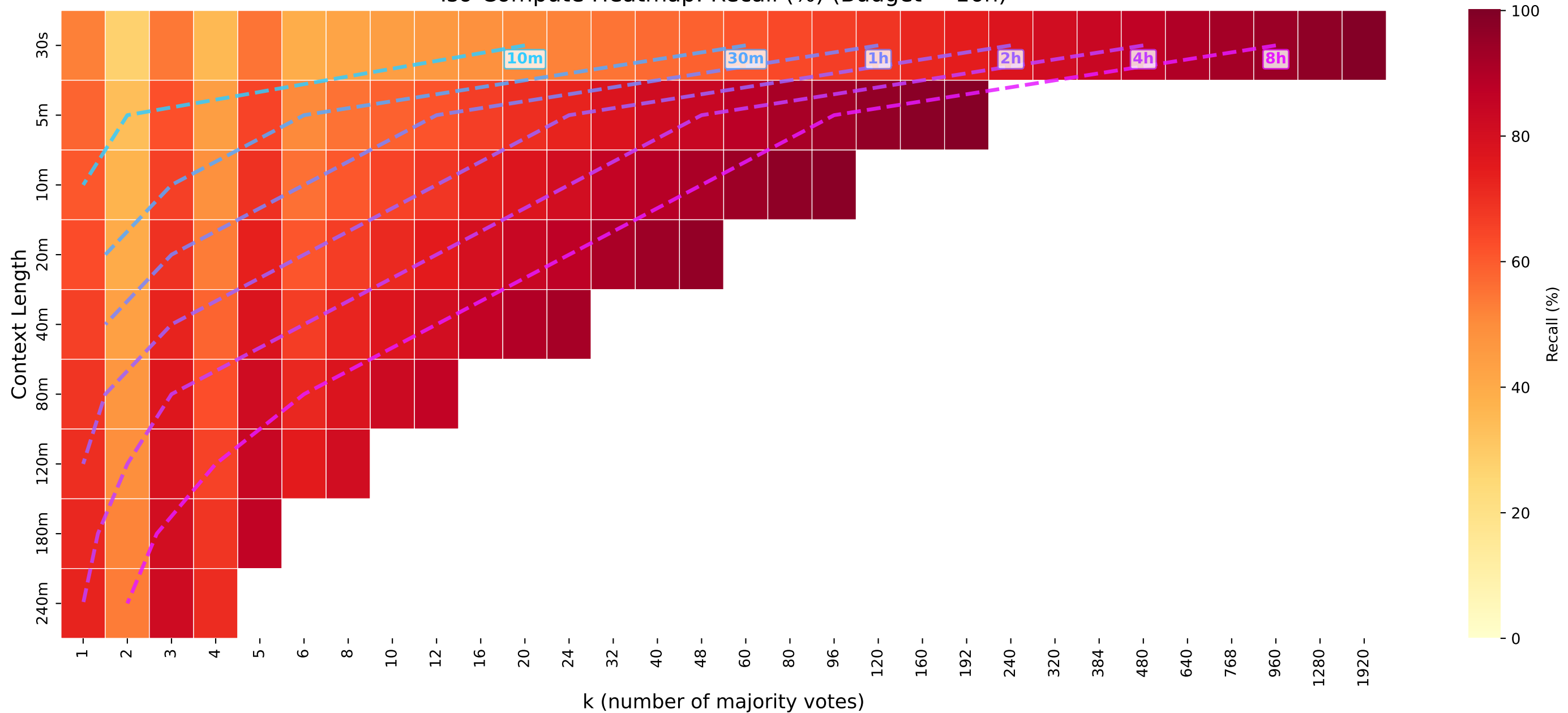
Iso-Compute Heatmap: Recall (%) (Budget = 16h)
