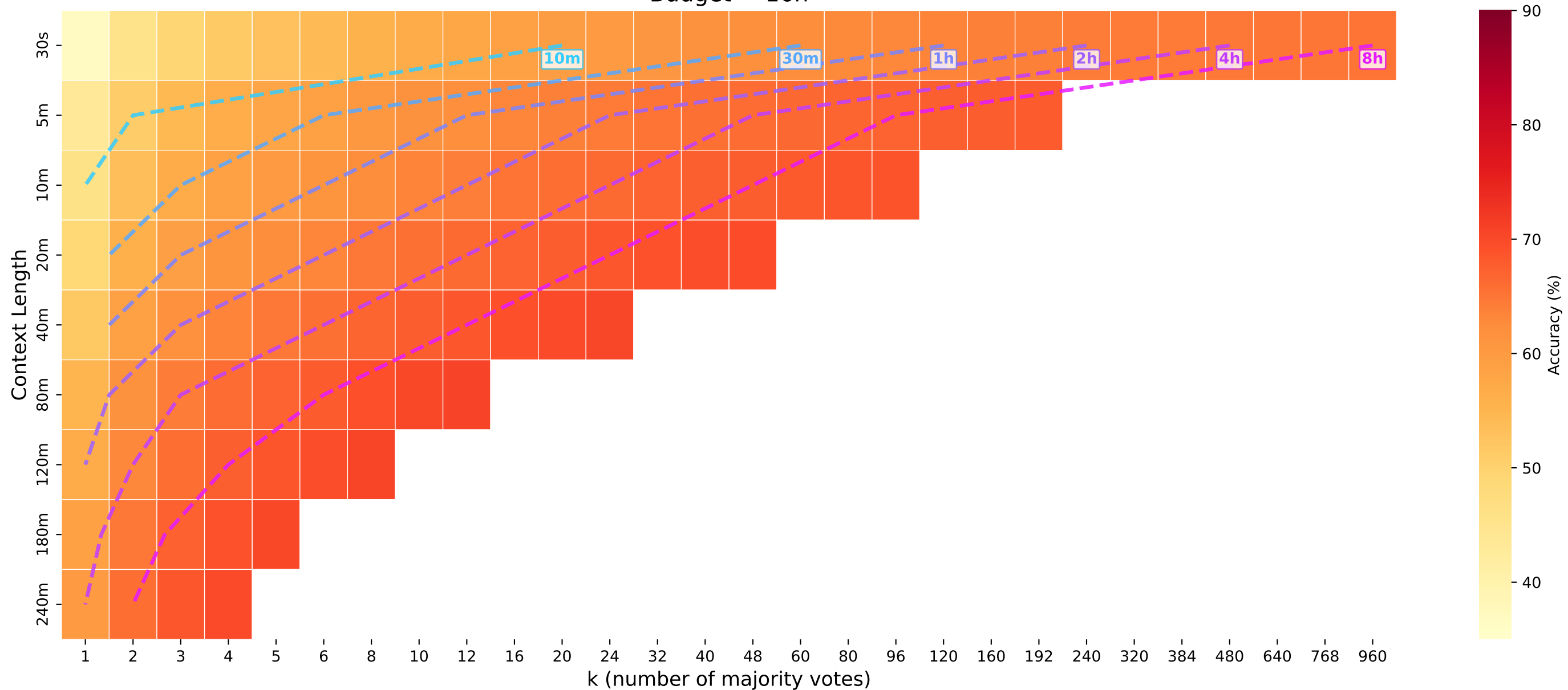
Iso-Compute Heatmap: Context Length vs Majority Voting (k) Budget = 16h
