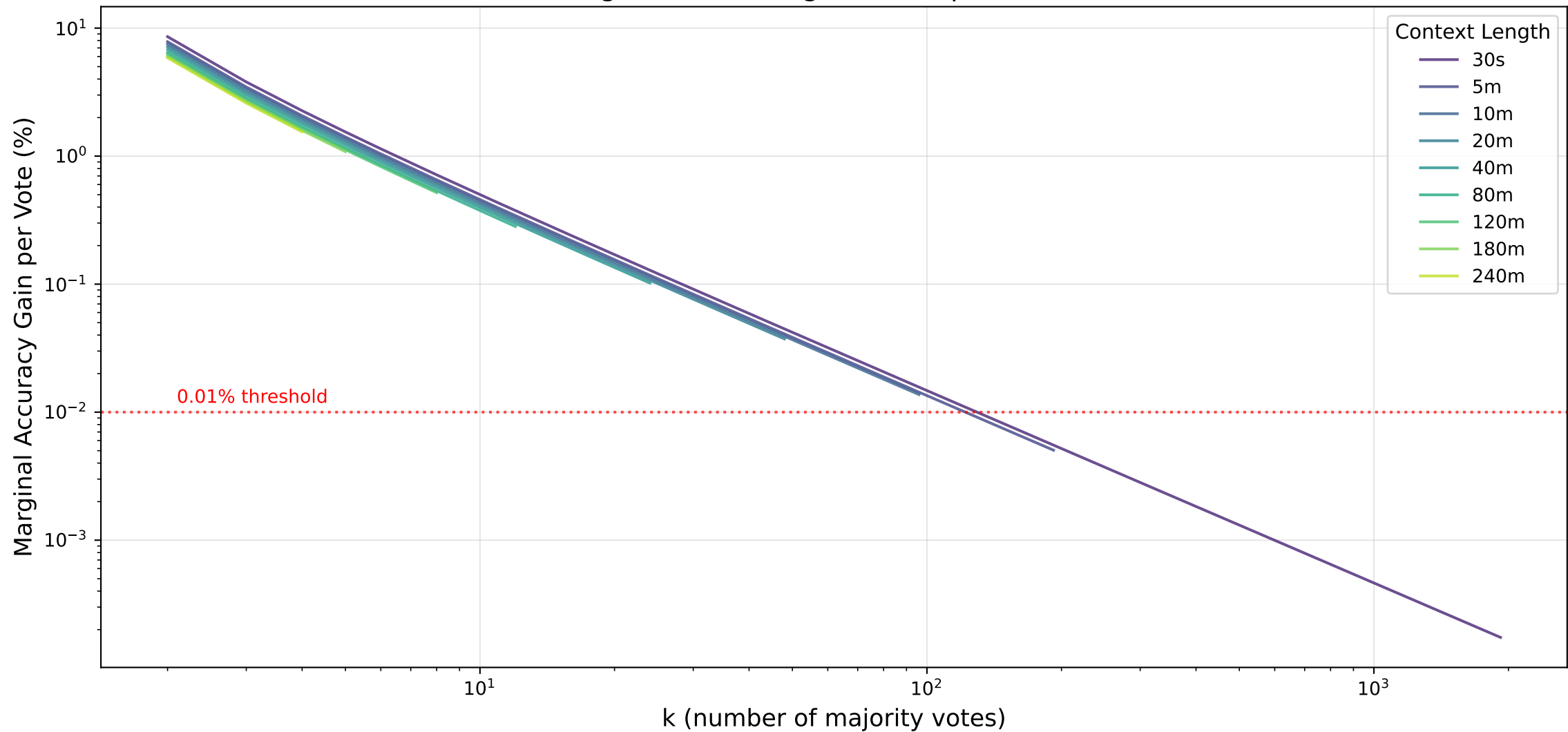
Diminishing Returns: Marginal Gain per Additional Vote
