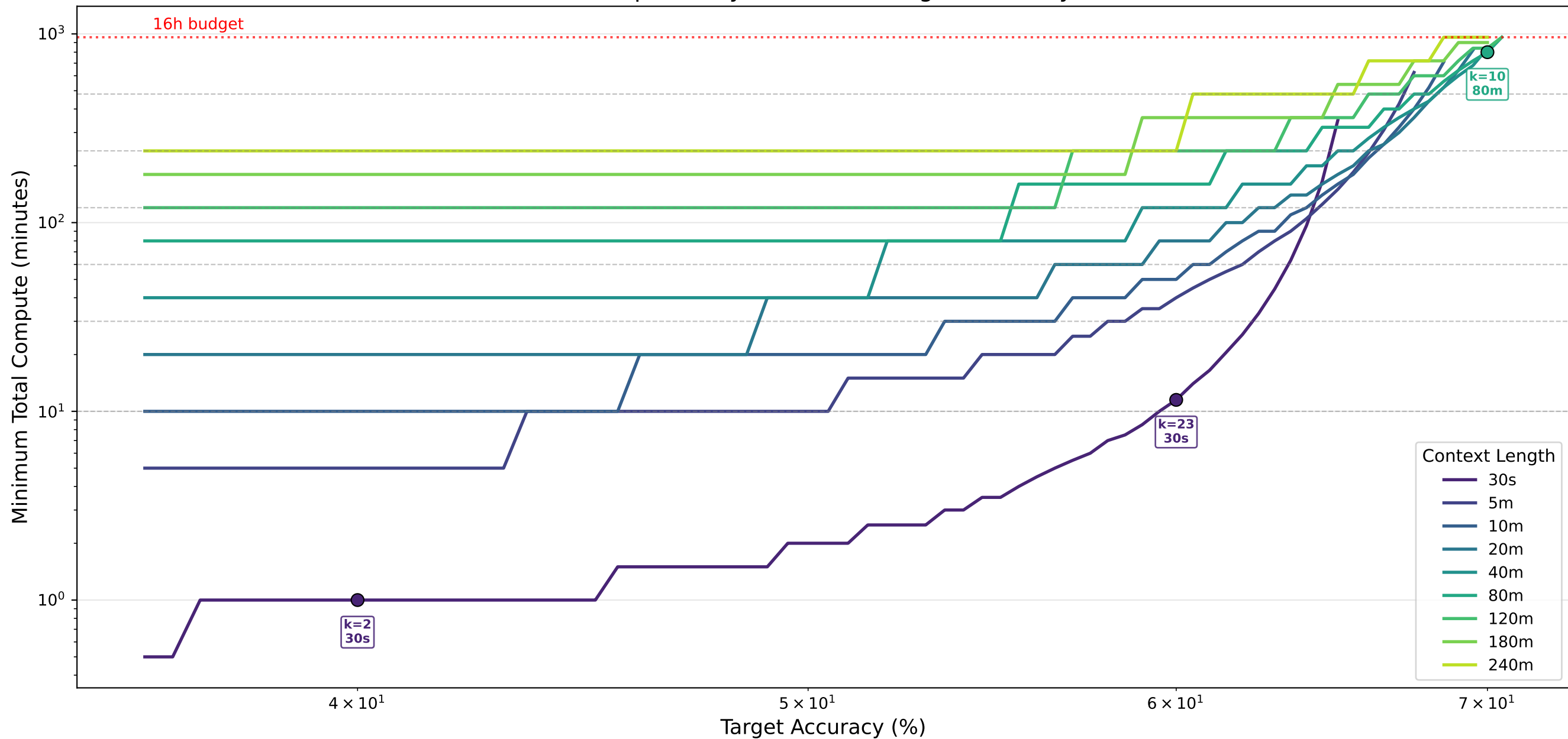
Cheapest Way to Reach a Target Accuracy
