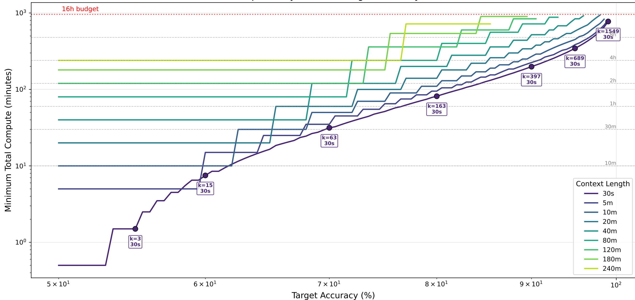
Cheapest Way to Reach Target Accuracy (%)
