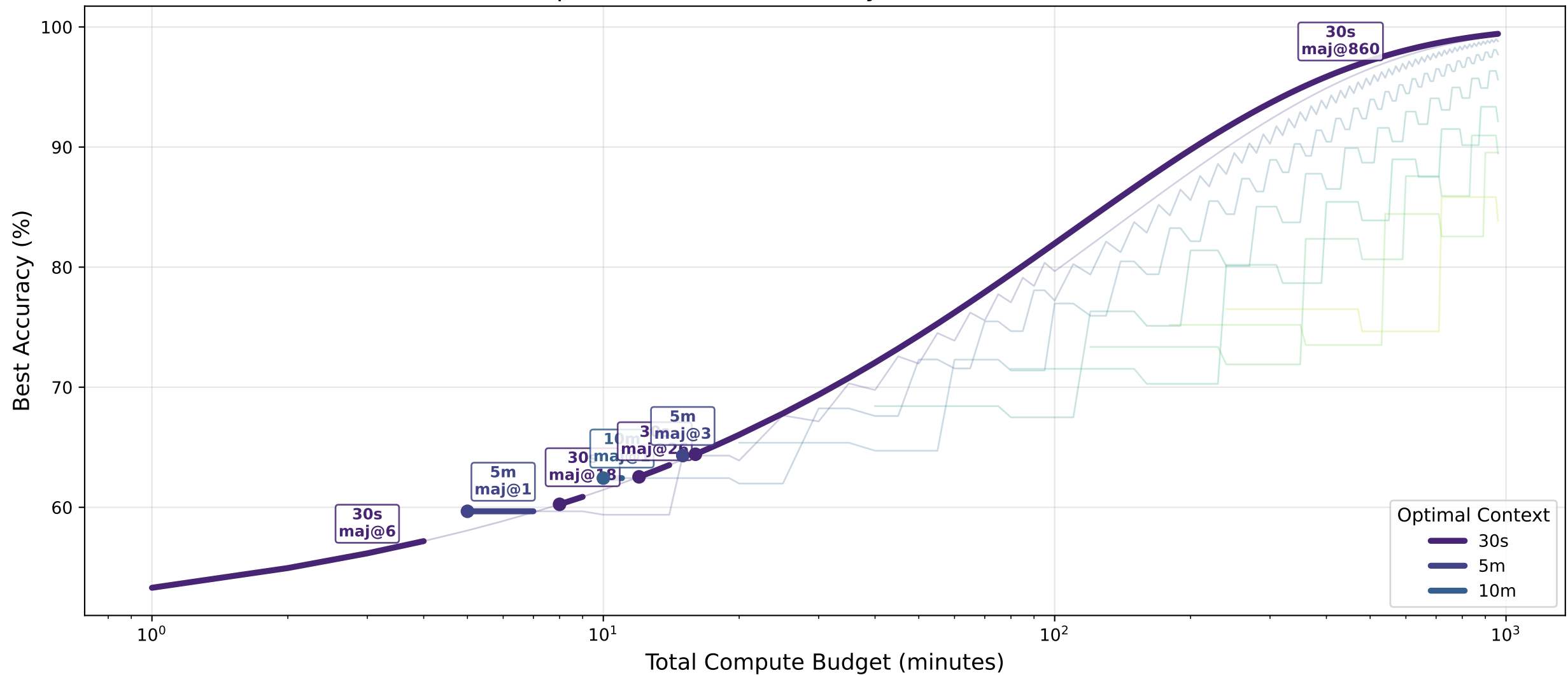
Optimal Tradeoff: Accuracy (%) (Pareto Front)
