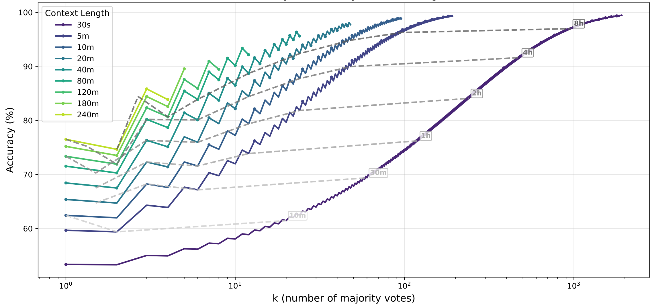
Accuracy (%) vs k by Context Length
