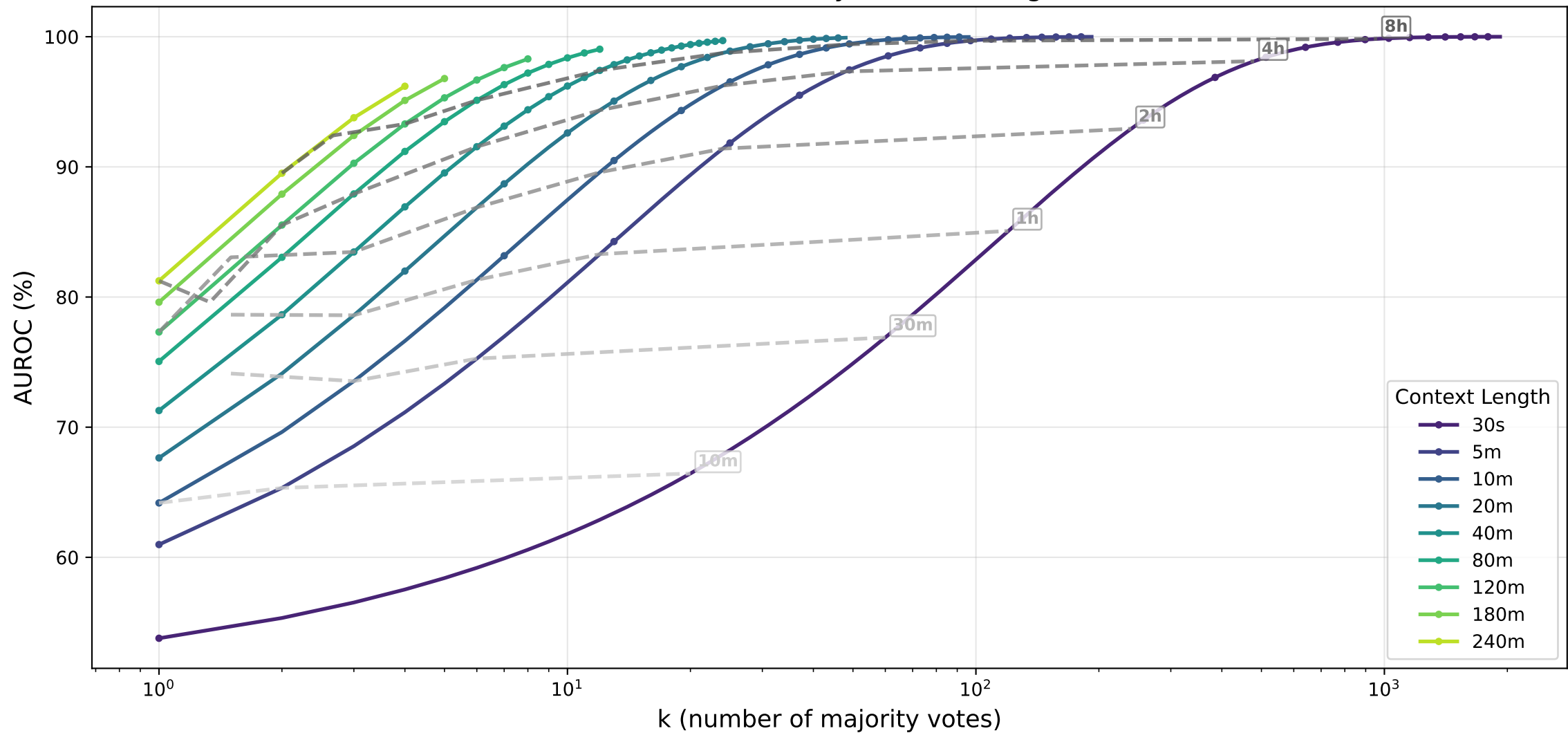
AUROC (%) vs k by Context Length
