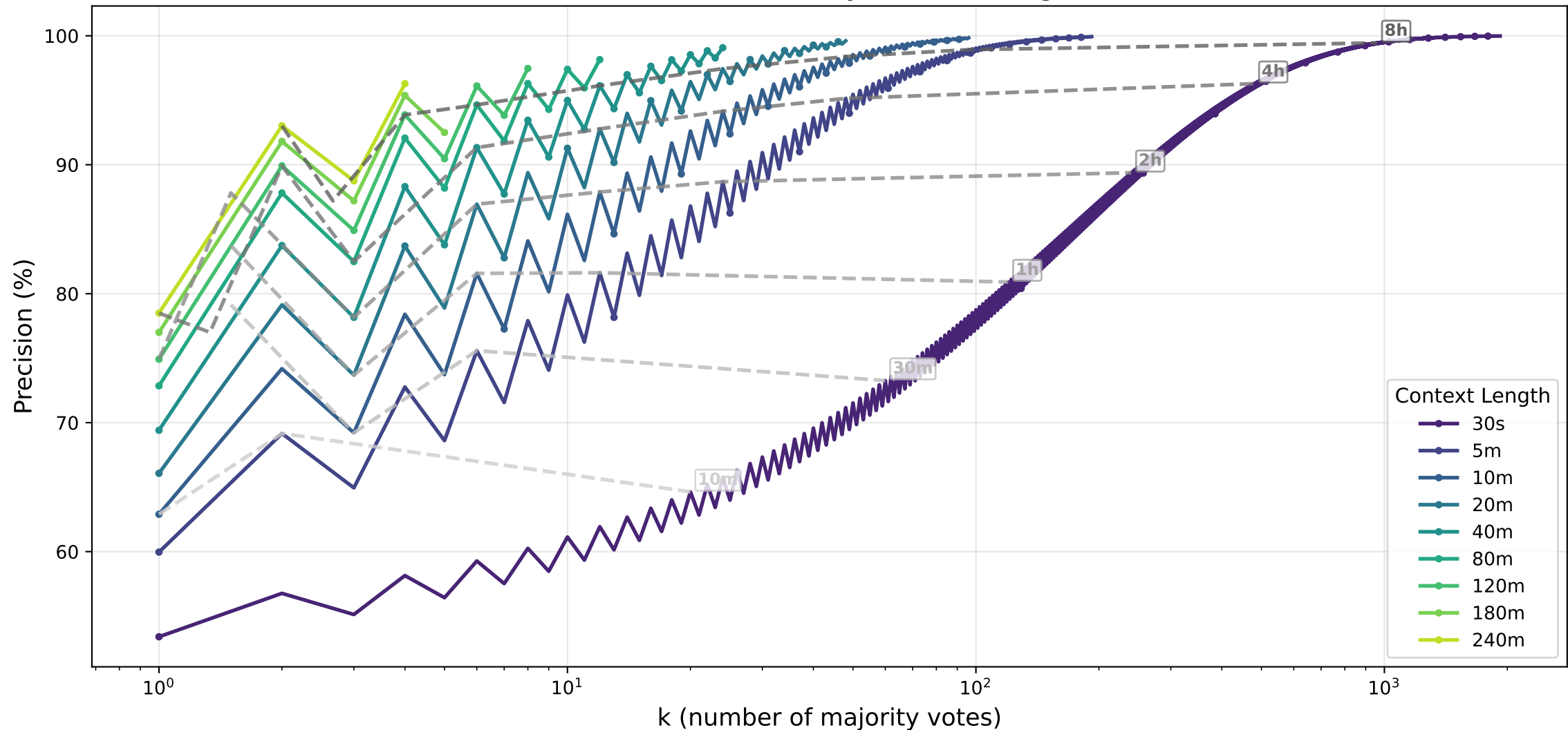
Precision (%) vs k by Context Length
