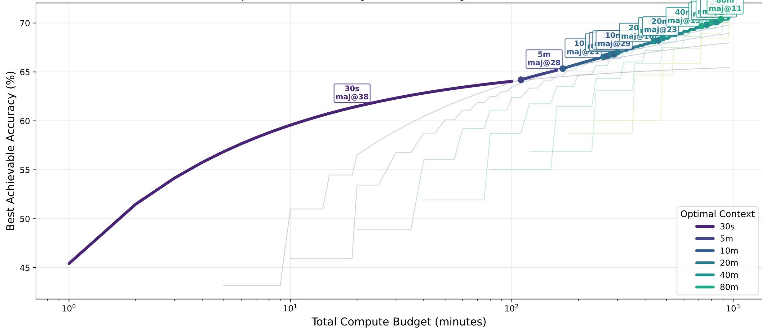
Optimal Context Length vs Total Budget (Pareto Front)
