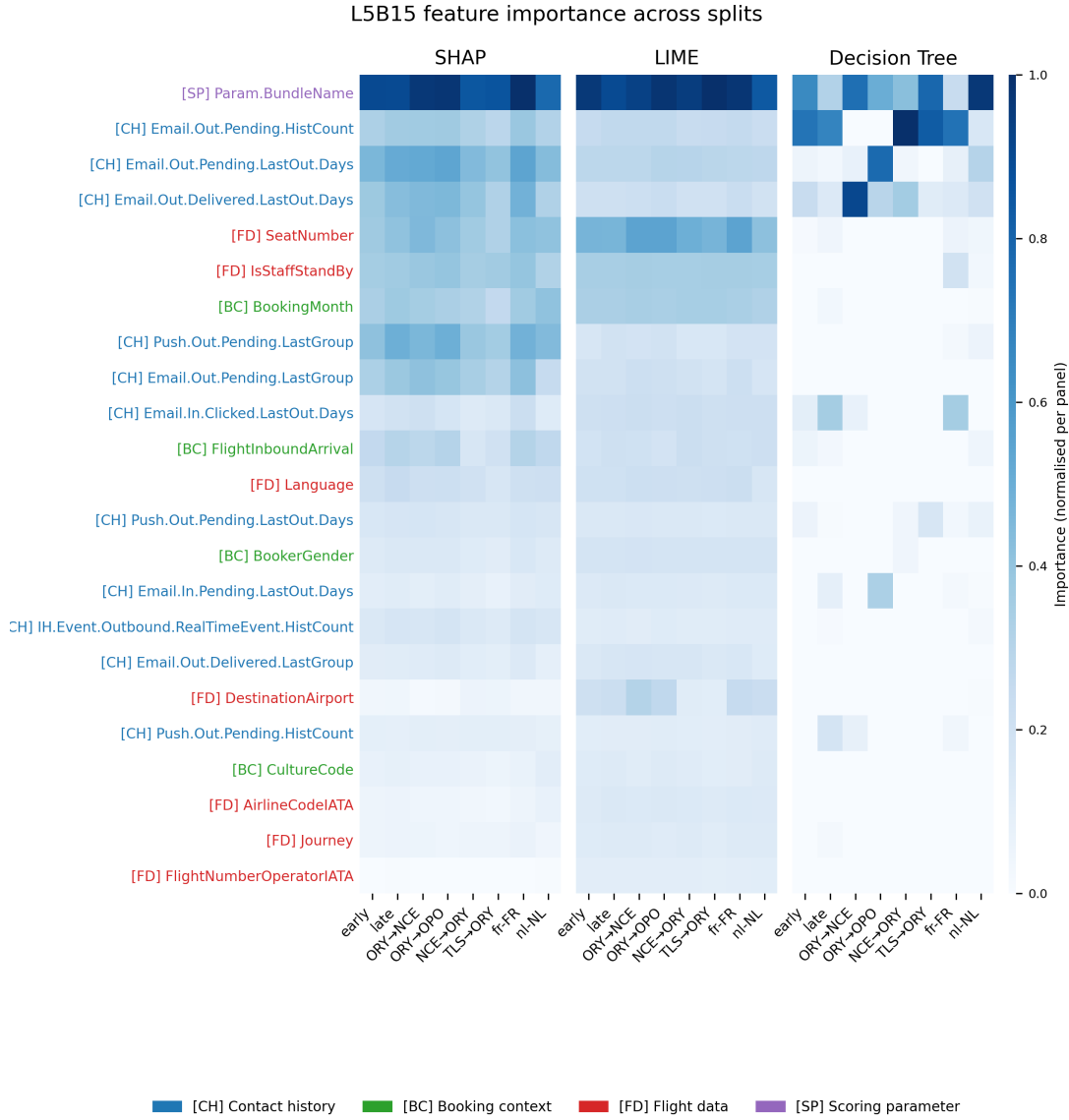
Figure 2: Normalised feature importance across L5B15 splits for SHAP, LIME, and the decision tree surrogate. Importance scores within each panel are normalised to [0, 1] by dividing by the panel maximum. Features are ordered by mean importance across all splits and methods, most important at top. Each feature is tagged by group: contact history, booking context, flight data, and scoring parameters.
