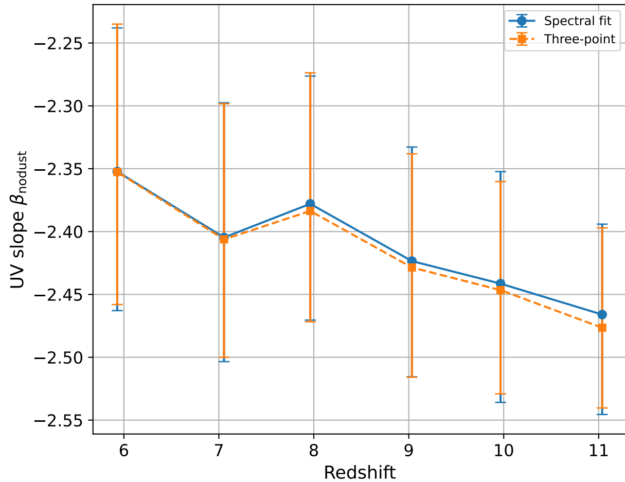
Evolution of \beta_{\text{nodust}}
