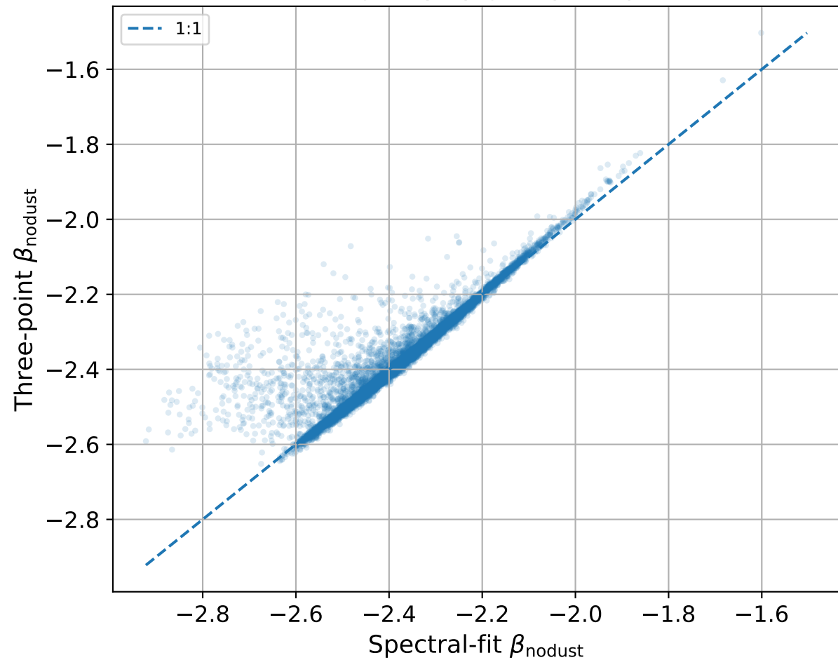
Dust-free galaxy-by-galaxy comparison
