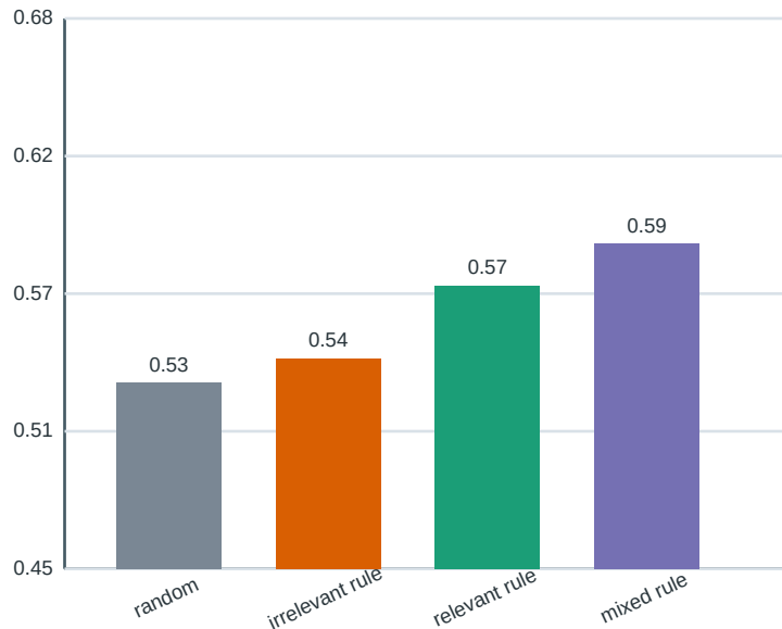
Transfer accuracy
