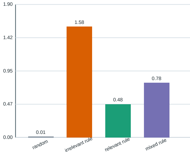
Learning-progress proxy
