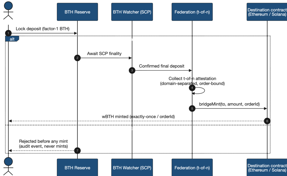
Figure 18: Wrap / lock \rightarrow mint flow (BTH \rightarrow wBTH). A factor-1 deposit is locked in the reserve, confirmed under SCP finality, attested by the federation to t -of- n , and minted on the destination chain against the deterministic orderId . A non-factor-1 deposit is rejected before any mint.
