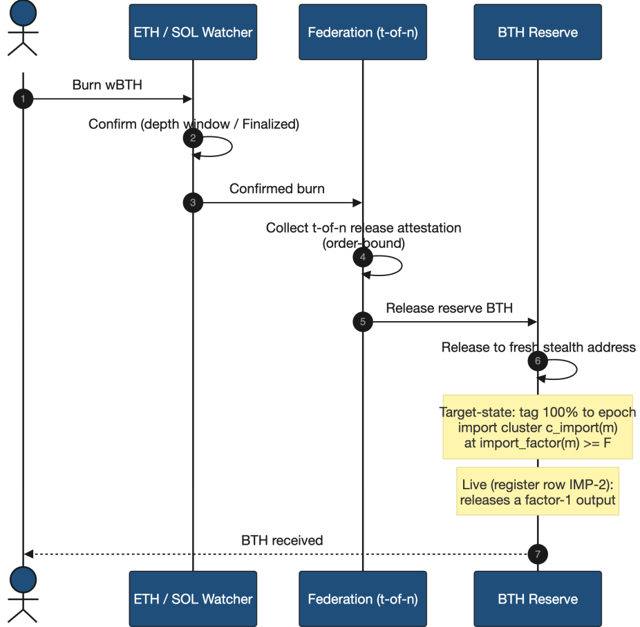
Figure 19: Unwrap \rightarrow import-tagging flow (wBTH \rightarrow BTH). A confirmed burn is attested and releases reserve BTH to a fresh stealth address, tagged 100% to the epoch import cluster c_{\text{import}}(m) at \text{import\_factor}(m) \geq F . Live as of protocol 5.0.0: the implementation tags the released output to the epoch import cluster at the elevated factor ( F = 1.5 \times \text{floor} , K = 1 day epoch; register row IMP-2).
