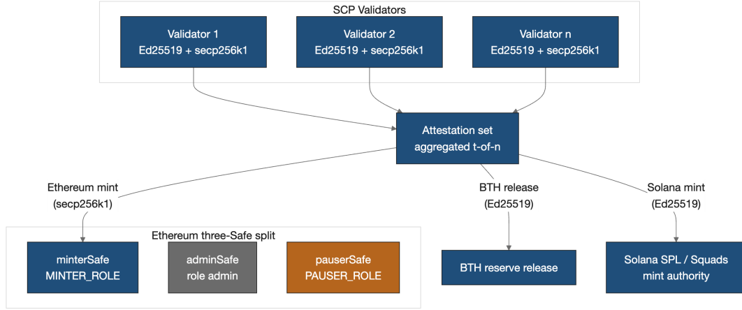
Figure 17: Federation custody and attestation topology. Each SCP validator operates an Ed25519 node key (BTH release + Solana mint) and a secp256k1 signer (Ethereum). Threshold envelopes are aggregated to t -of- n and consumed by the mint / release paths; the Ethereum authority is a three-Safe split.
