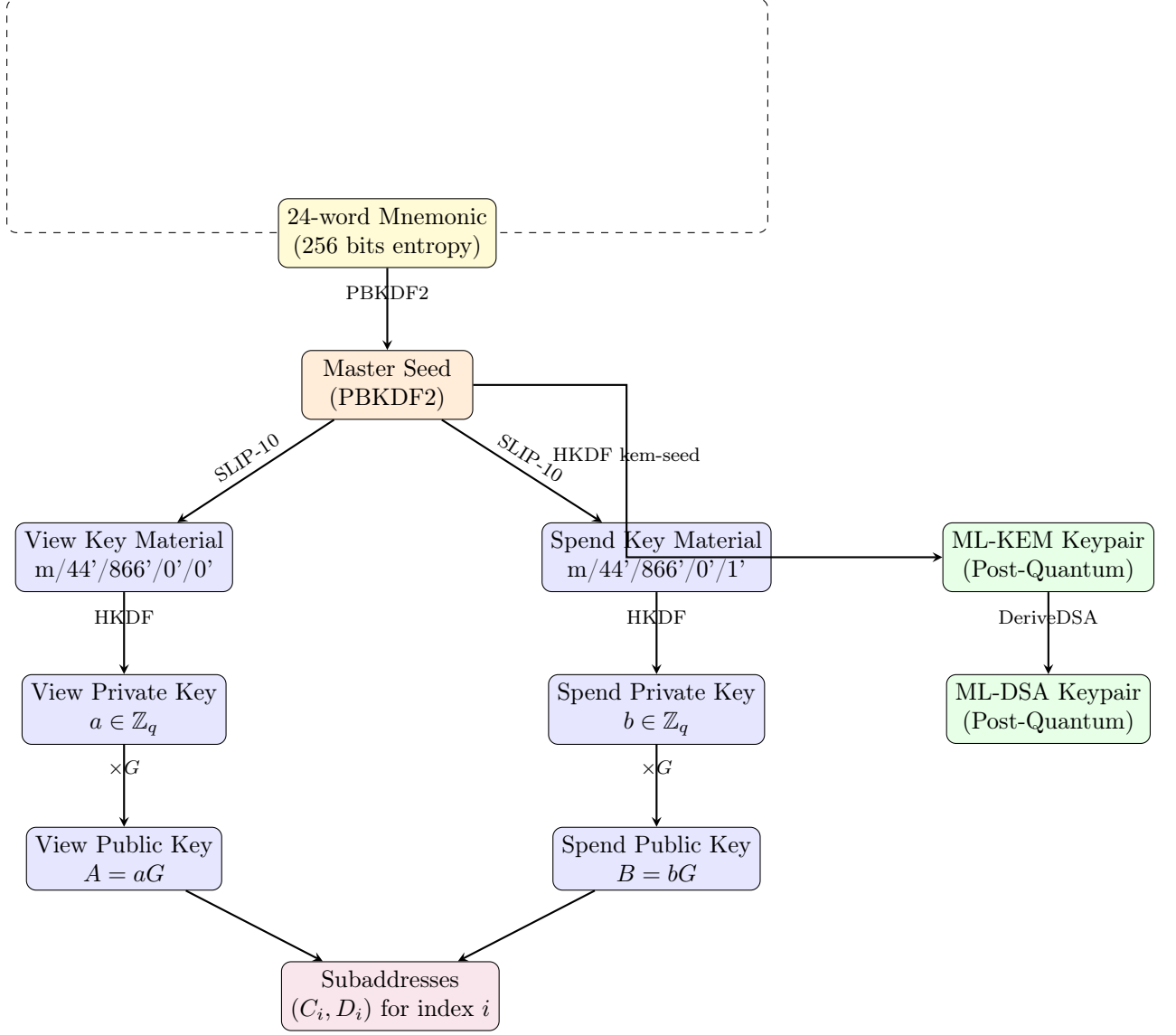
Figure 1: Key derivation hierarchy. A single BIP39 mnemonic derives all keys via SLIP-10 paths and HKDF domain separation. Classical Ristretto255 keys support ring signatures, while post-quantum ML-KEM/ML-DSA keys protect recipient privacy and minting operations.
