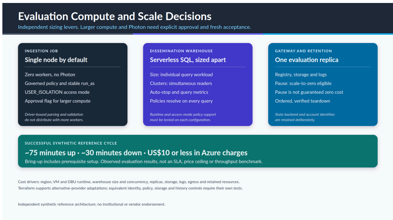
Figure 10 — Scalability & Compute Strategy: ingestion and dissemination compute can be sized independently while preserving the configured policy model.
