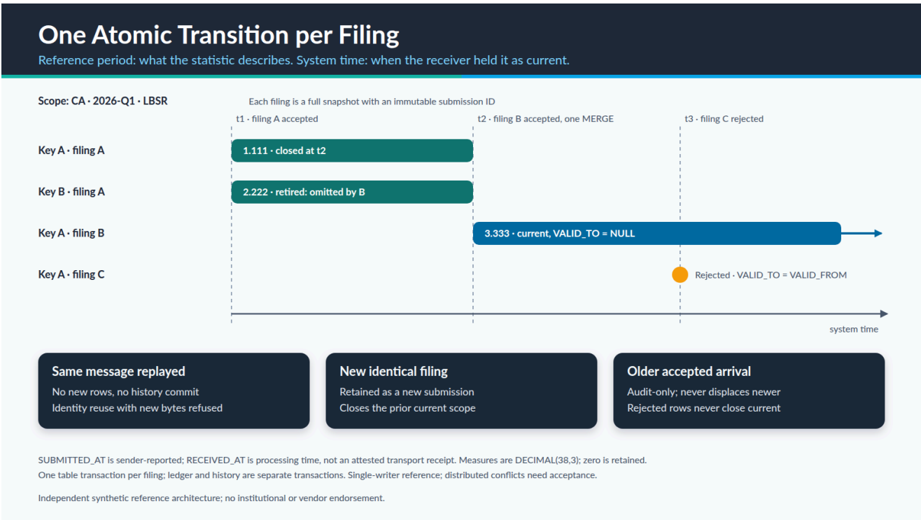
Figure 9 — Temporal SCD2 Delta Merge: accepted revisions update the current state; rejected revisions remain audit-only and preserve the last accepted observation.
