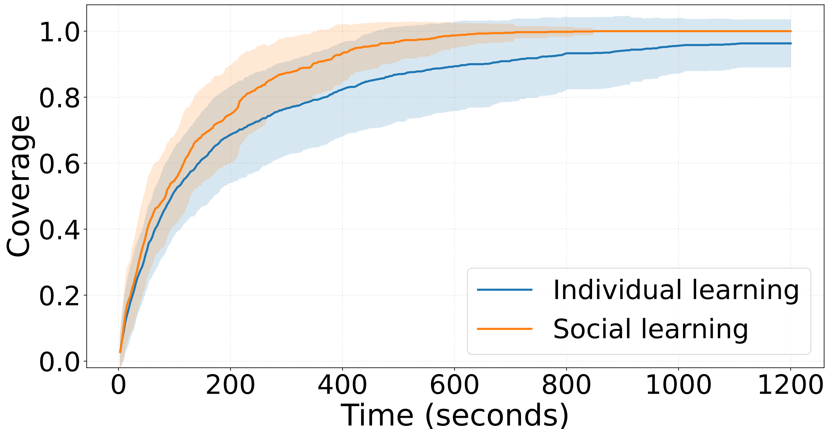
Individual vs. social learning on baseline environment
