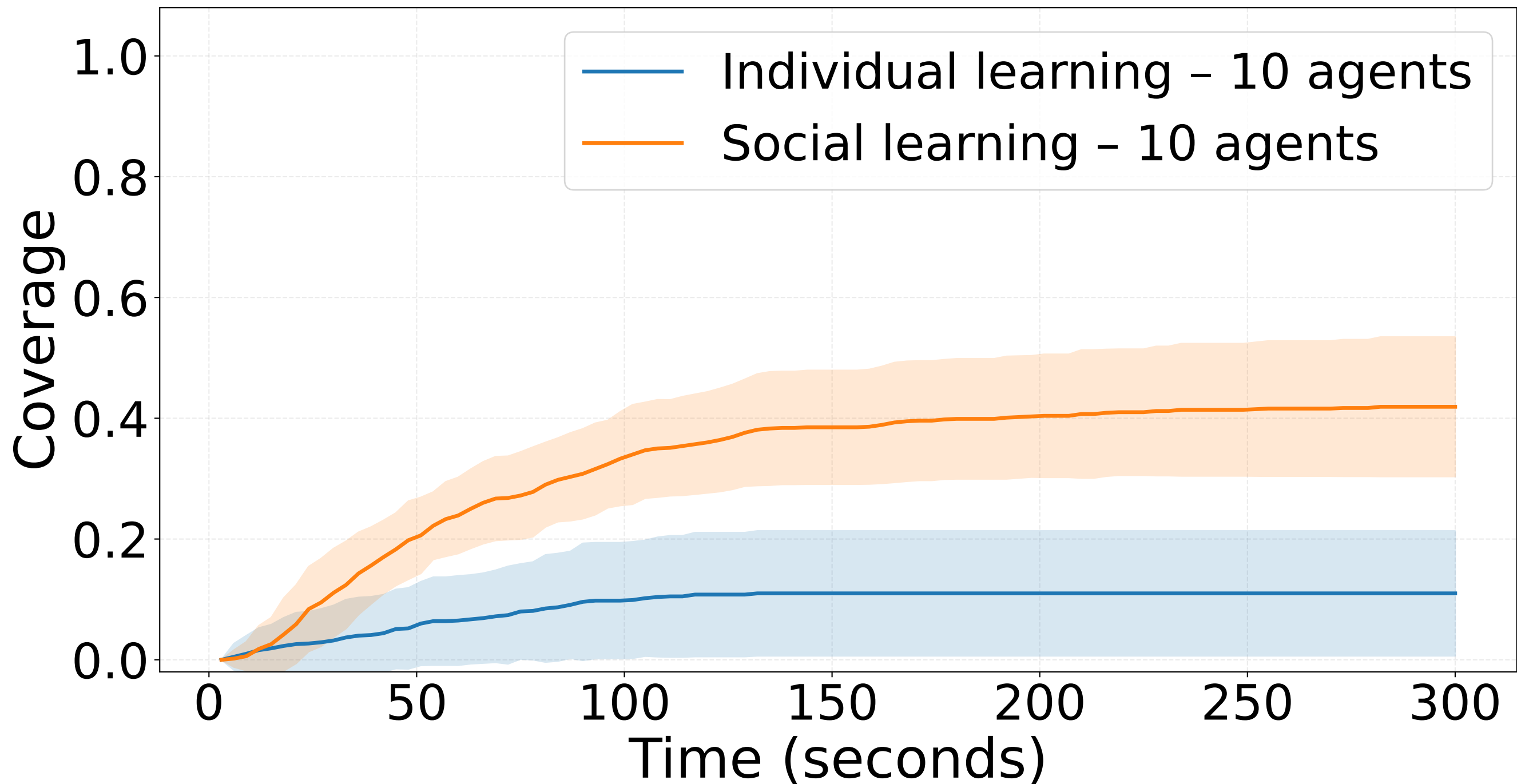
Individual vs. social learning on non-re-emission environment with 10% information
