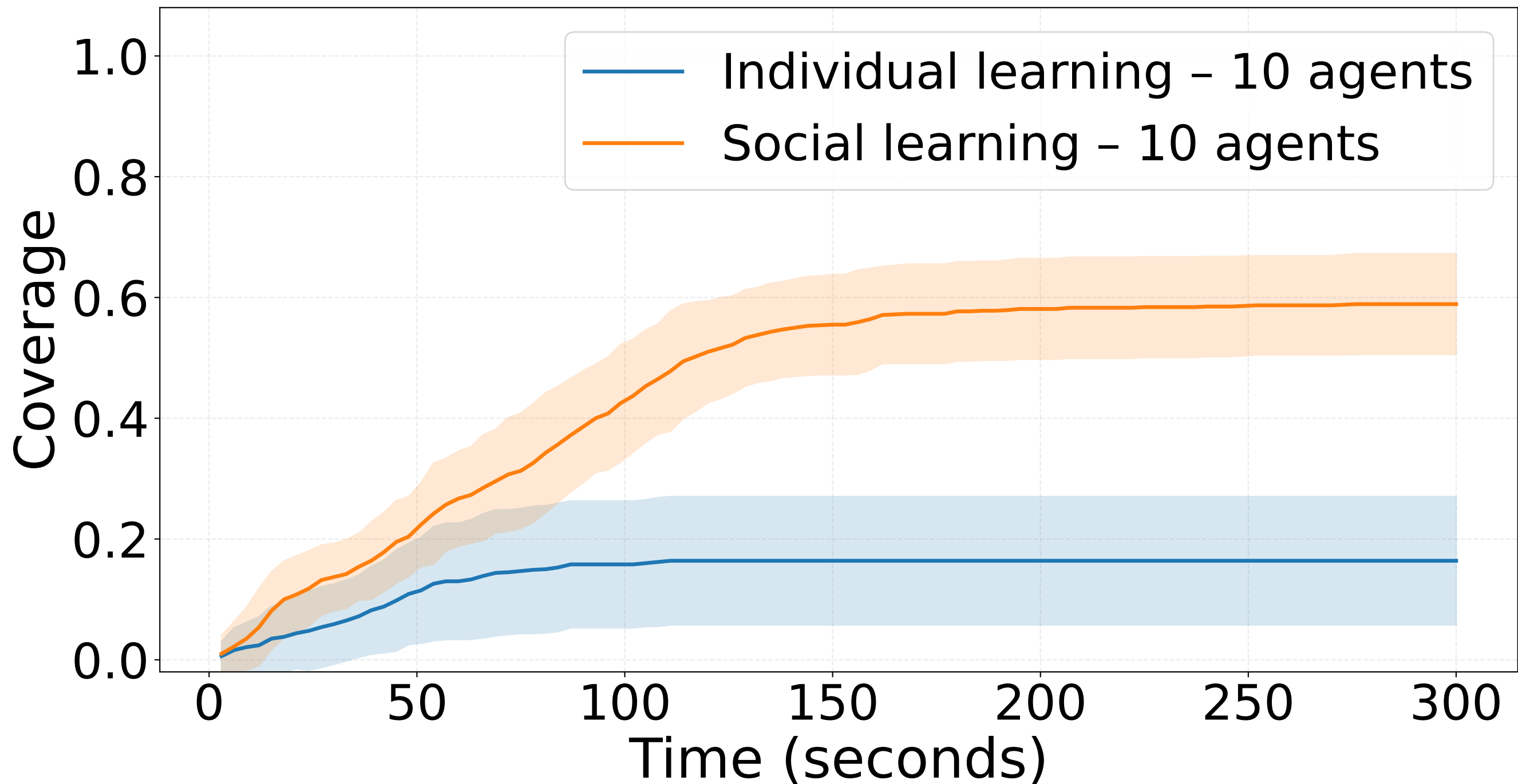
Individual vs. social learning on non-re-emission environment with 20% information
