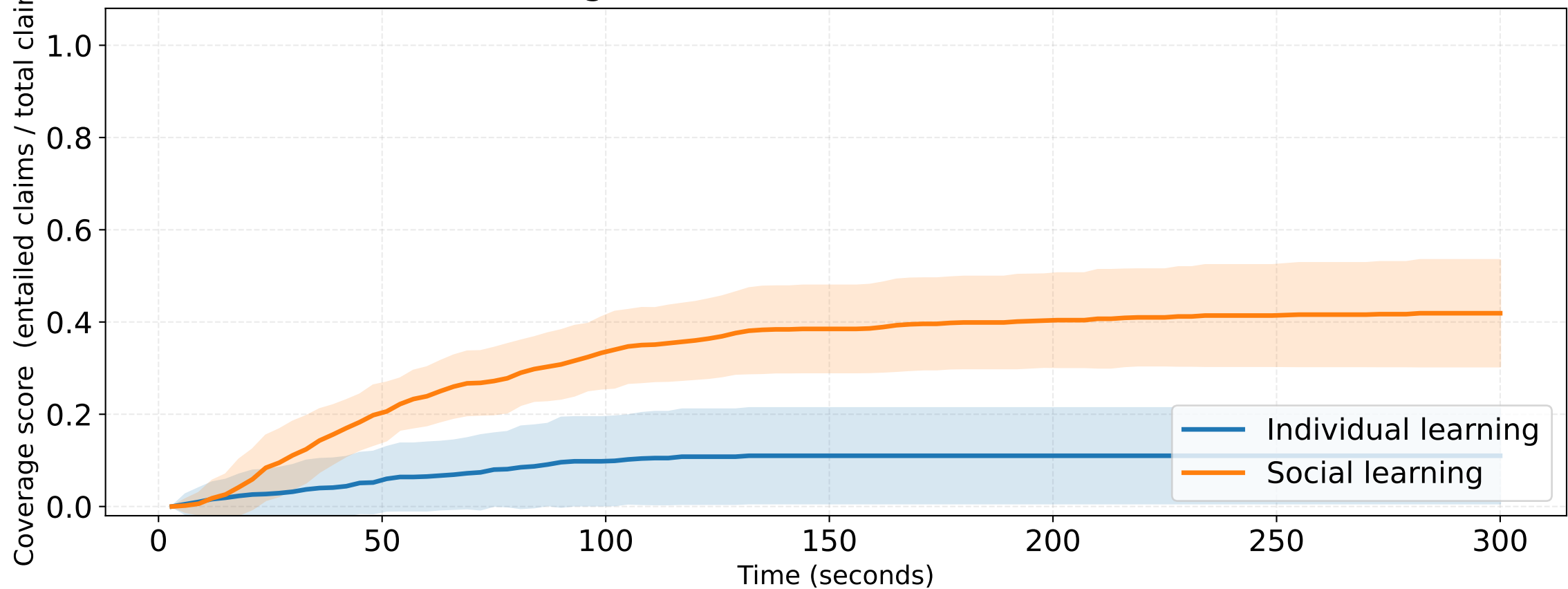
Individual vs. social learning on non-remission environment with 10% information
