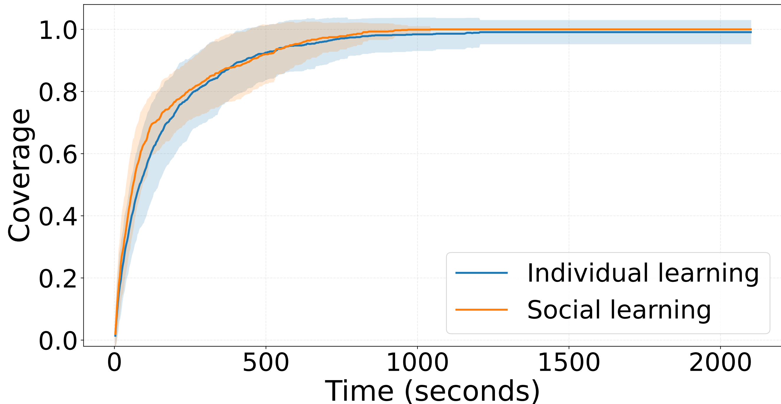
Individual vs. social learning on re-emission environment with 80% information
