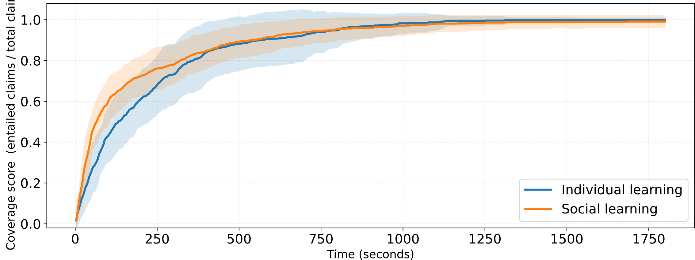
Individual vs. social learning on re-emission environment with 50% information
