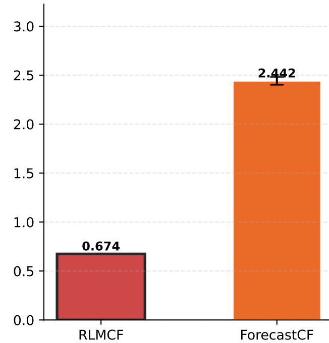
Proximity L2 ↓
