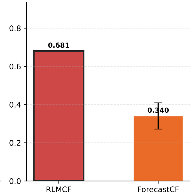
Compactness ↑
