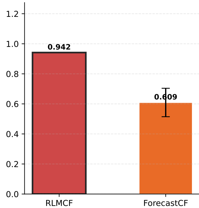
Validity Ratio ↑
