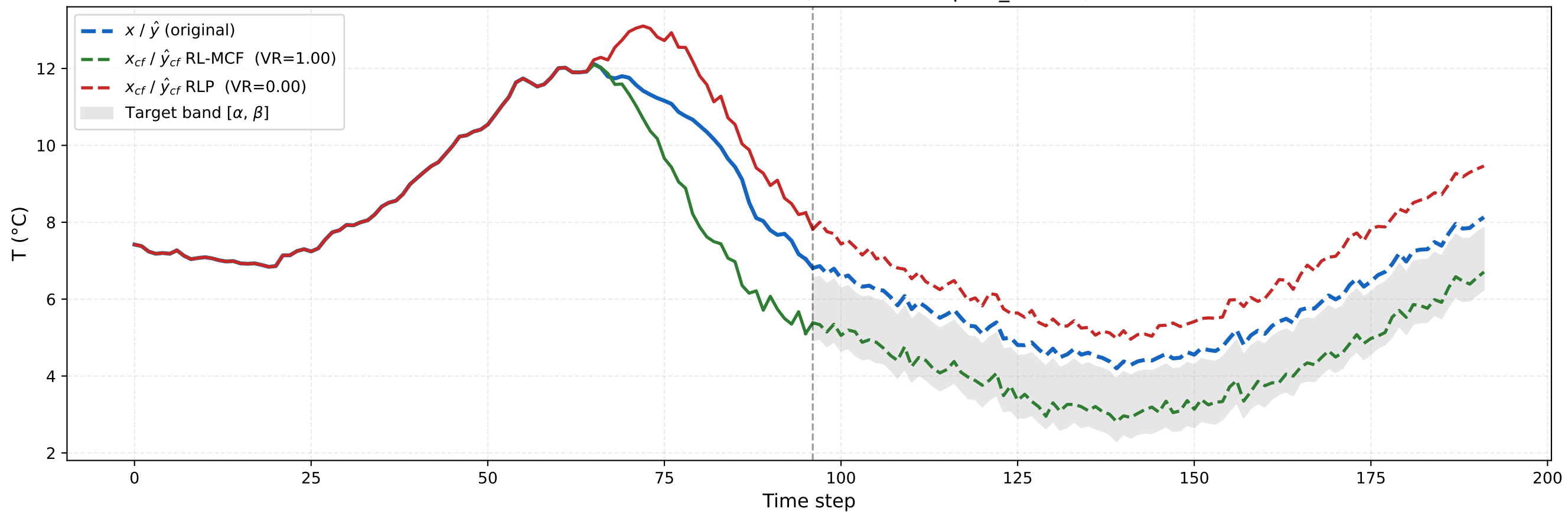
Weather — RL-MCF vs RLP (iTransformer, pred_len=96)
