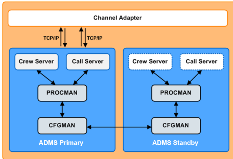
Figure 1. High Availability Design
