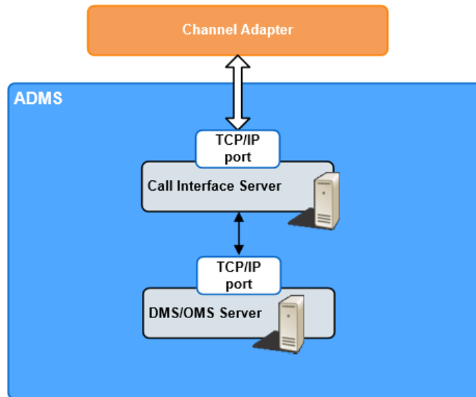
Figure 25. ADMS Components
