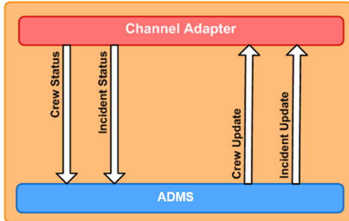
Figure 9. Message Convention
