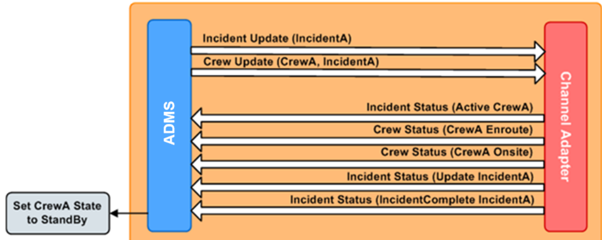
Figure 11. Simple Assignment
