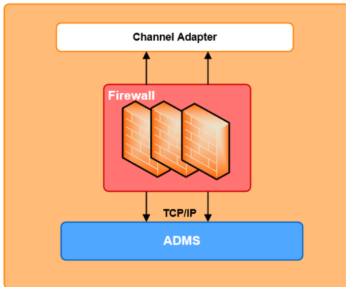
Figure 2. Firewall
