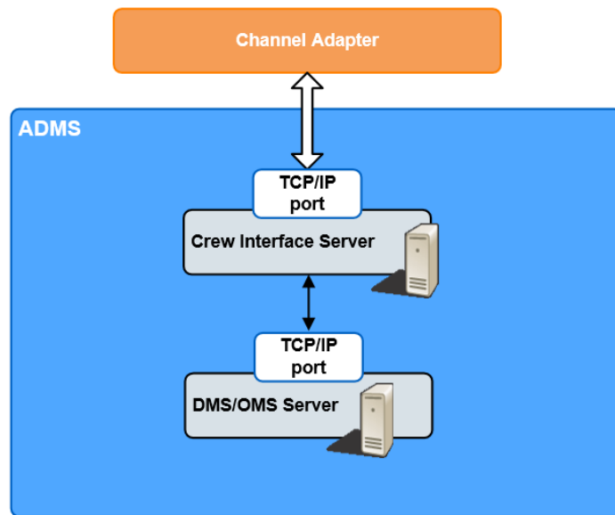
Figure 8. ADMS Components
