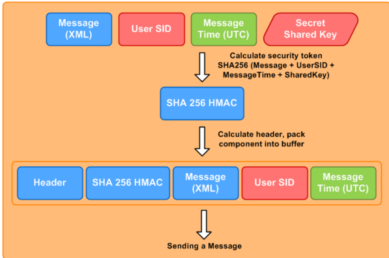
Figure 4. Sending a Message
