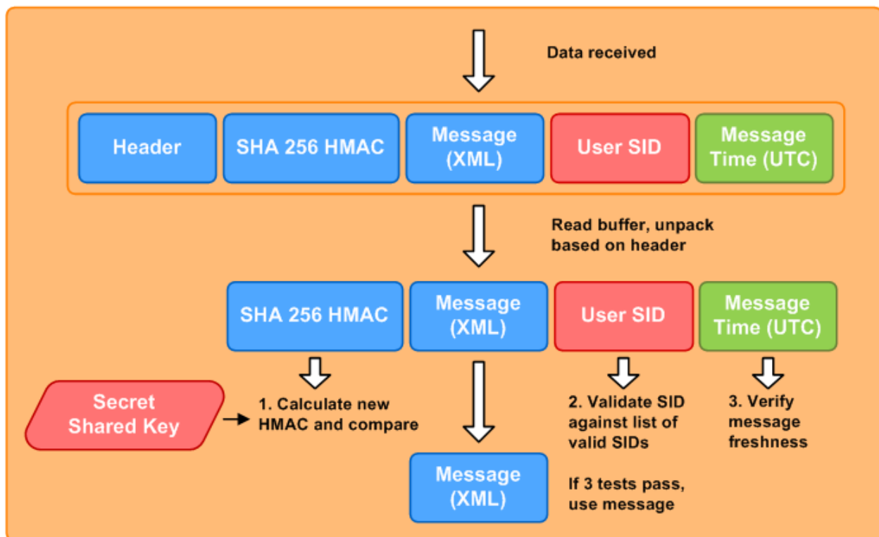
Figure 5. Receiving a Message
