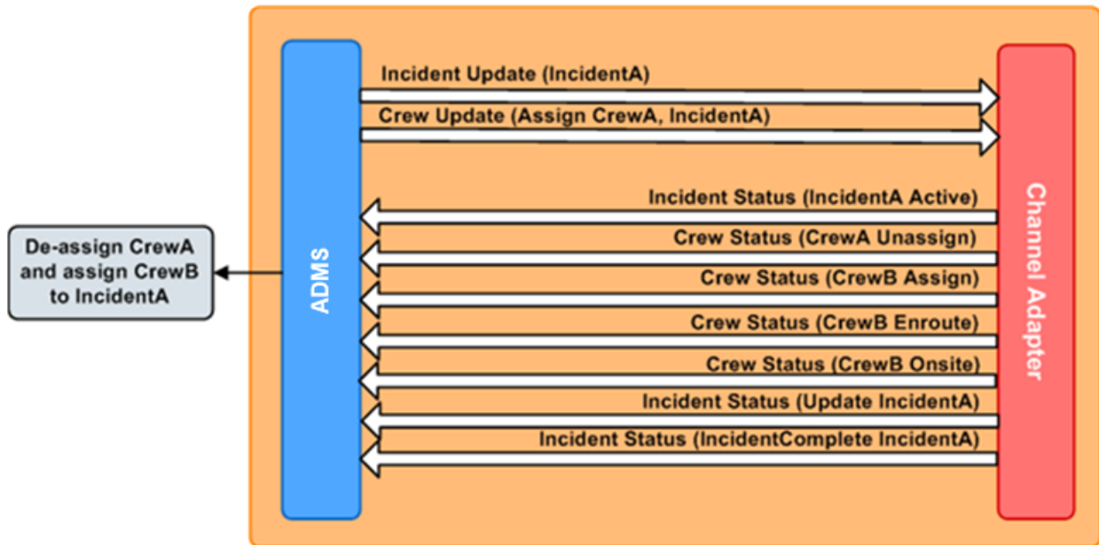
Figure 14. Order Re-Assignment by WFM
