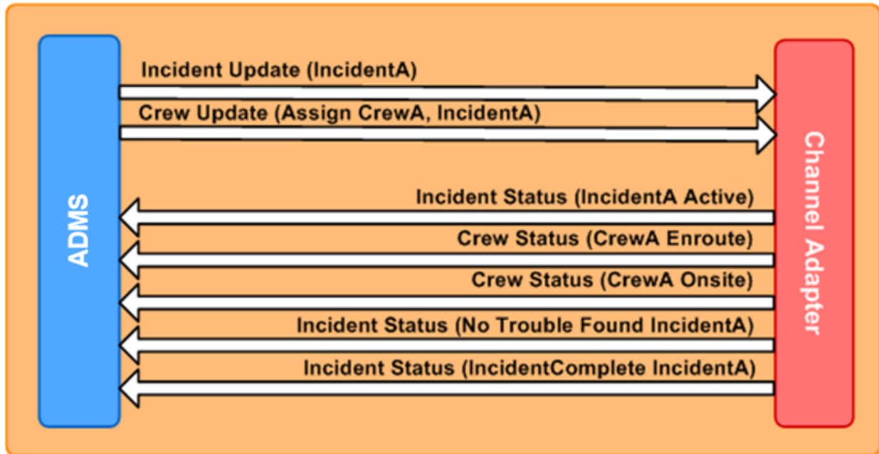
Figure 12. No Trouble Found
