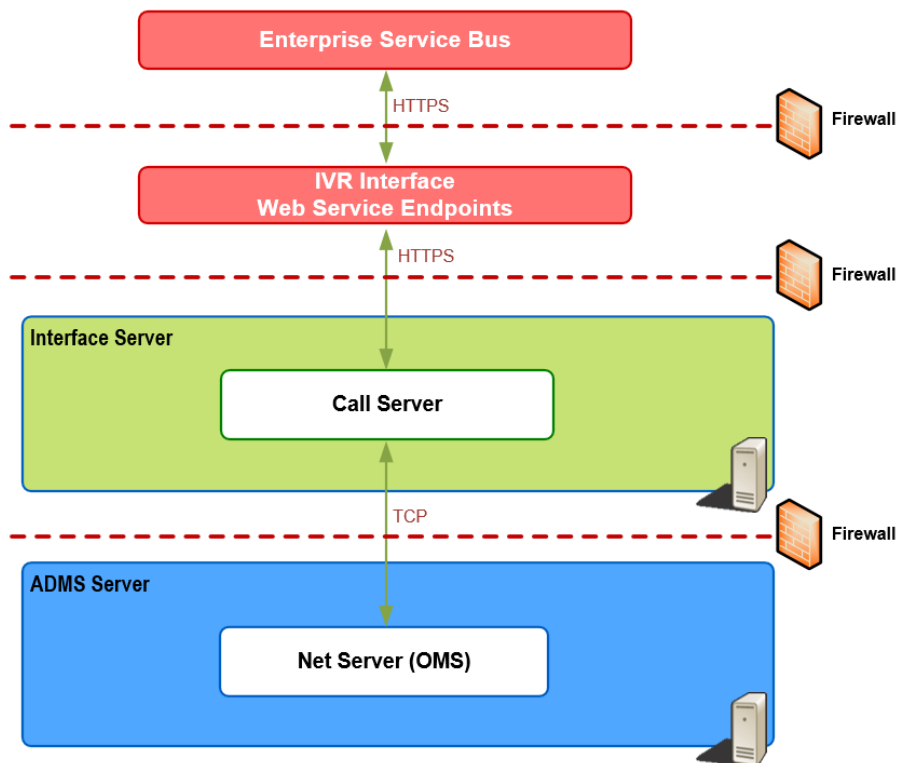
Figure 28. ADMS-IVR Data Flow
