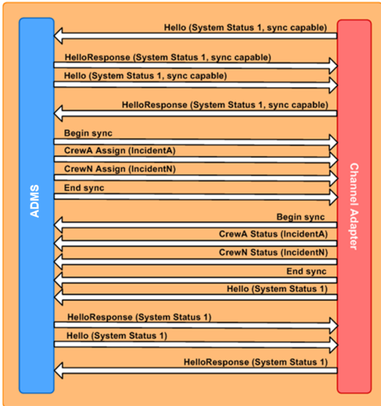
Figure 10. Hello Messages
