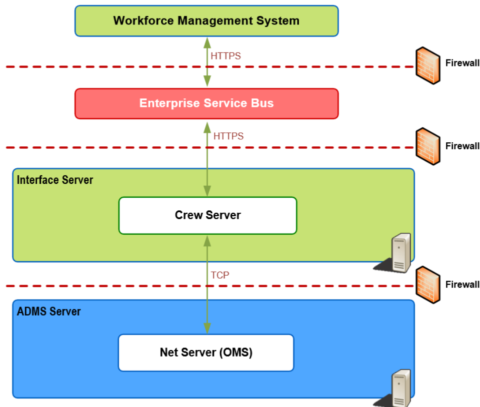
Figure 27. ADMS-WFM Data Flow
