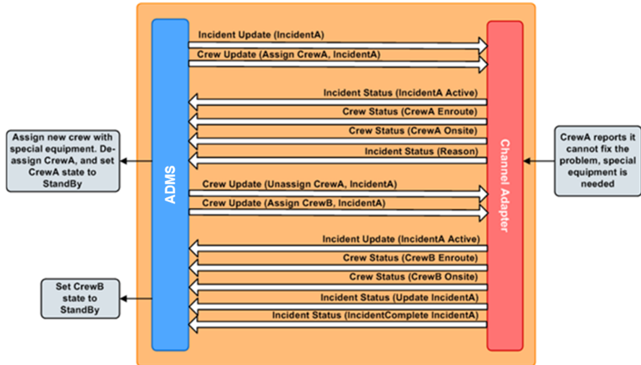
Figure 13. Order Re-Assignment by ADMS
