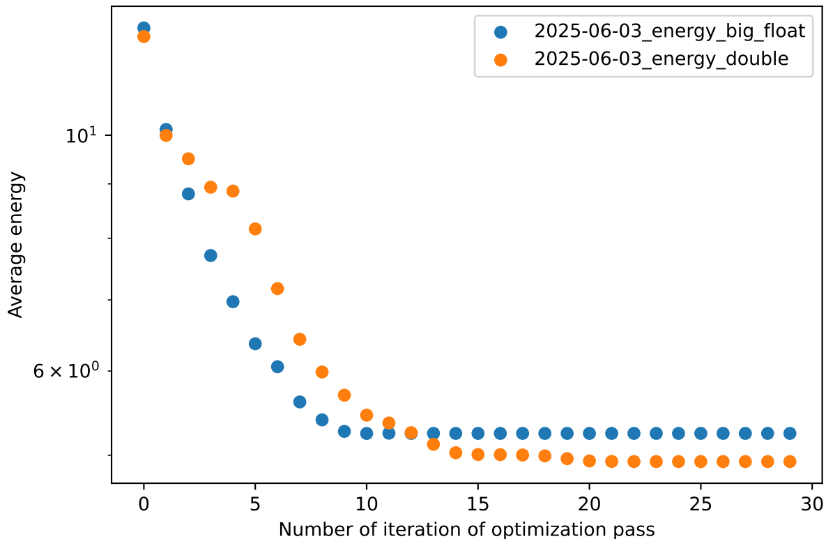
Average energy across all the model according to the number of optimization pass
