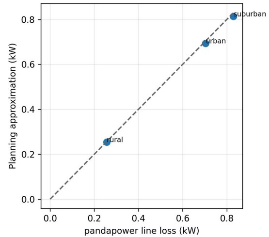
Fig. 5. All-AC approximation versus pandapower at the benchmark operating point.
