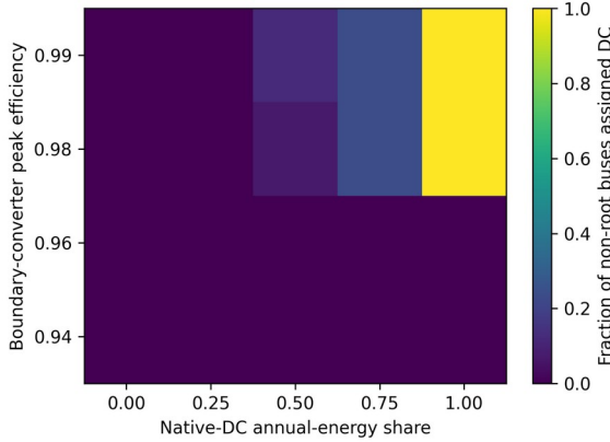
Fig. 3. Suburban architecture transition under K3; values are bus fractions assigned DC.
