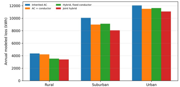
Fig. 2. Matched decomposition of annual modeled losses under the central setting.
