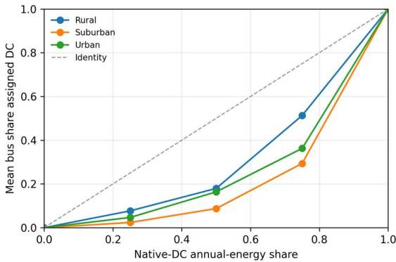
Fig. 4. Mean DC-assigned bus share versus native-DC energy share at 98% efficiency.
