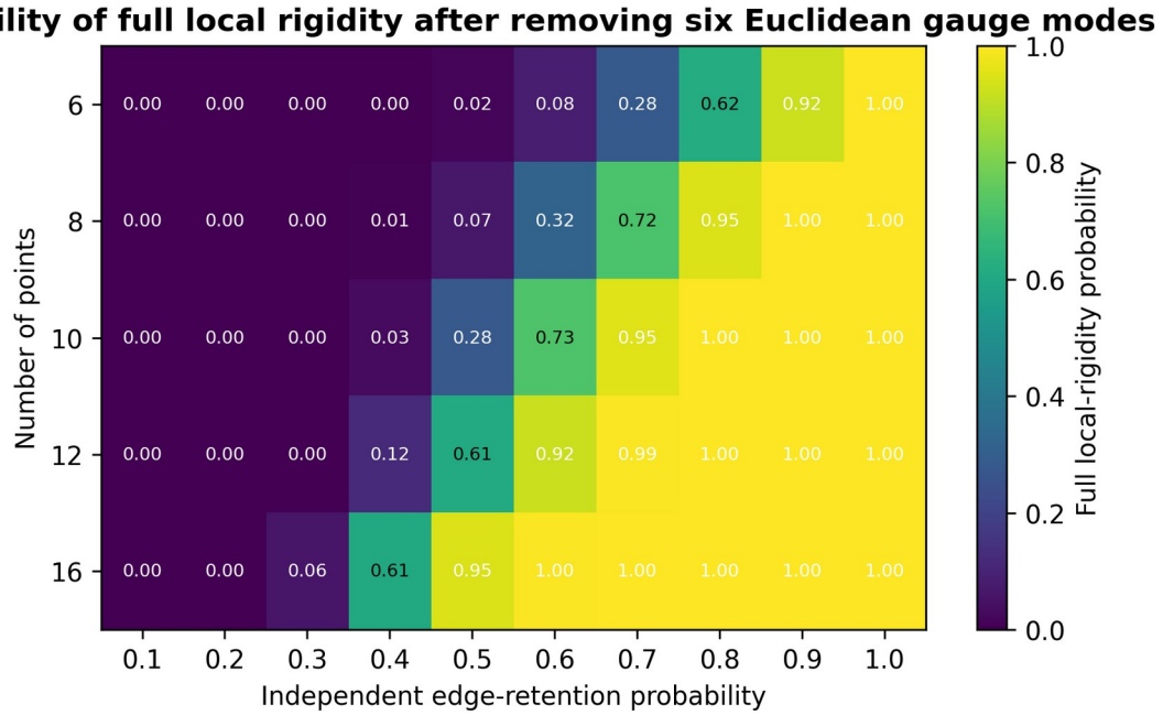
Fig. 4 Probability of full local rigidity for generic three-dimensional random frameworks. Each cell summarizes 2000 independently sampled point-and-edge realizations after the six infinitesimal Euclidean gauge modes are removed. The result concerns local rigidity, not global uniqueness.
