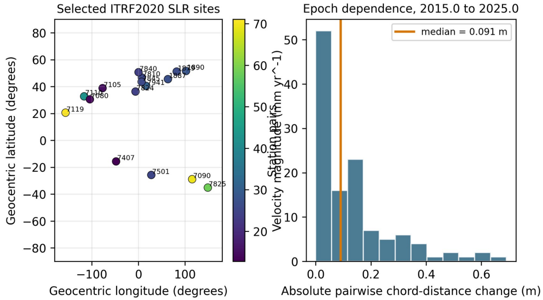
Fig. 5 ITRF2020 demonstration. The left panel shows the selected SLR sites and published velocity magnitudes. The right panel shows absolute pairwise Euclidean chord-distance changes after linear propagation from epoch 2015.0 to 2025.0; this is an epoch-sensitivity calculation, not a reflected physical realization.
