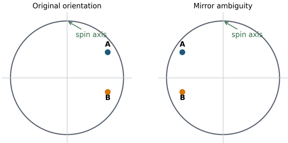
Signed longitude is pairwise on the principal branch; poles and antipodes are undefined
