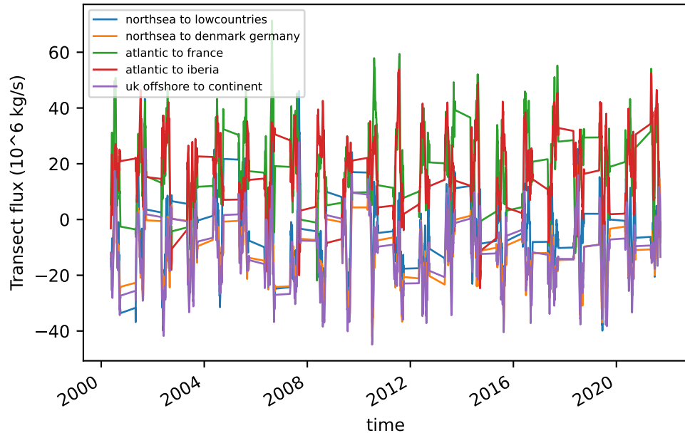
(b) Cross-transect moisture flux (30d mean)
