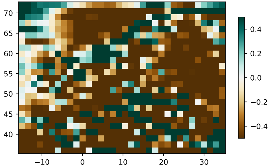
(a) Mean MFC (kg m -2 day -1 )
