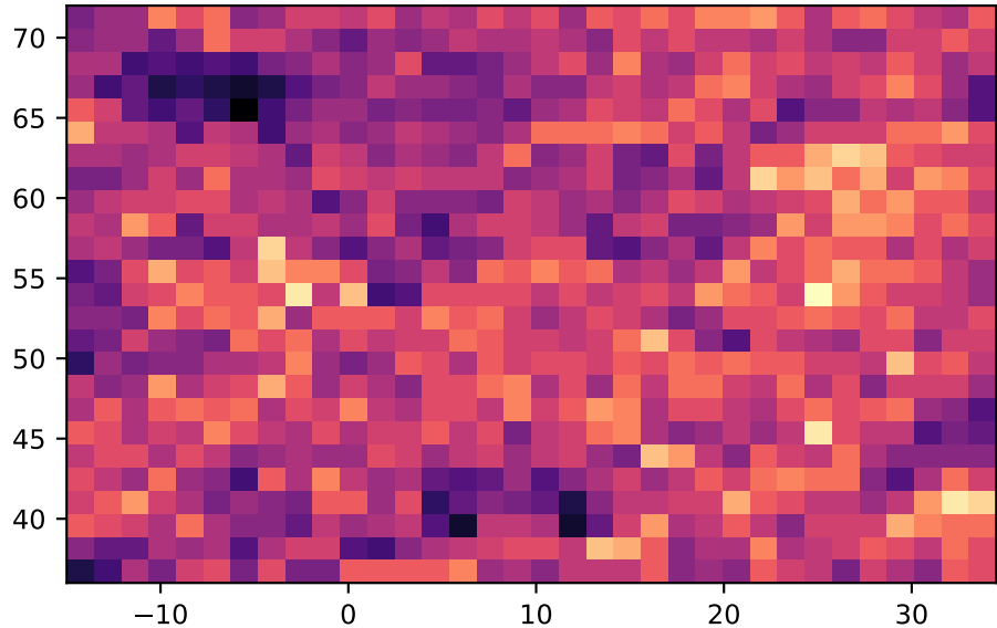
(a) Event count per cell (2000-2021)
