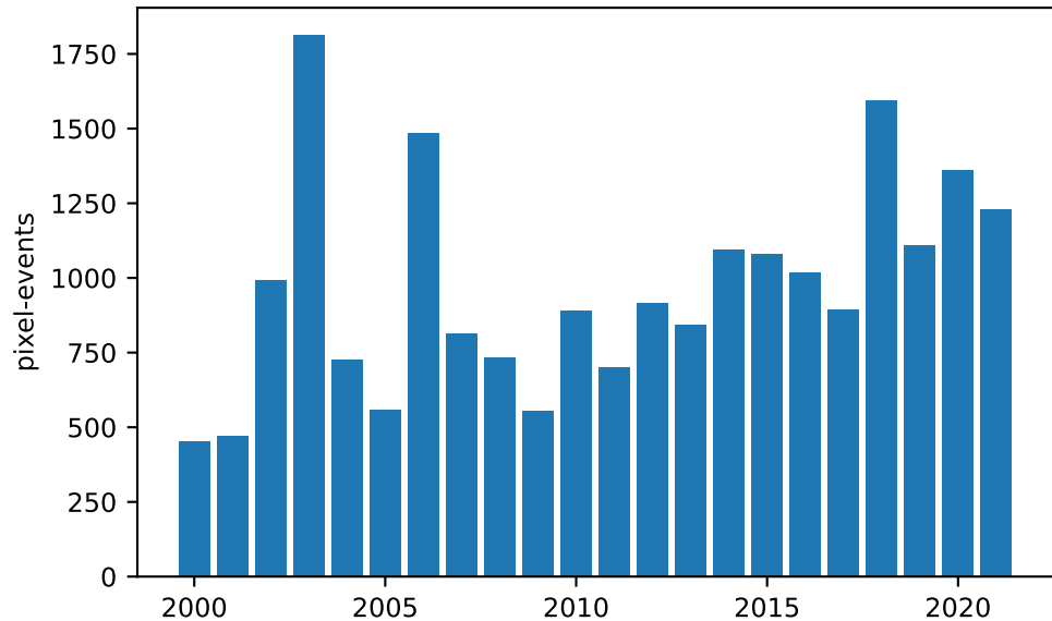
(b) Events per year (primary def)
