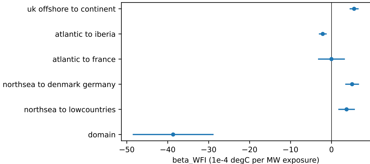
(c) Panel effect of upstream deployment on Tmax anomaly
