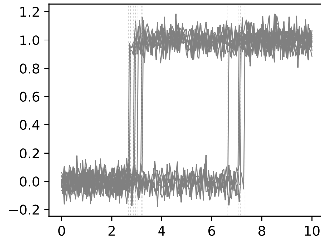
Two clusters: unit curves
