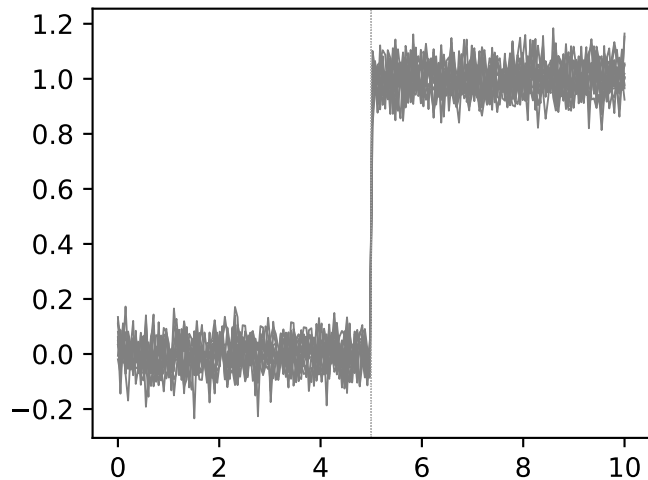
Synchronous: unit curves
