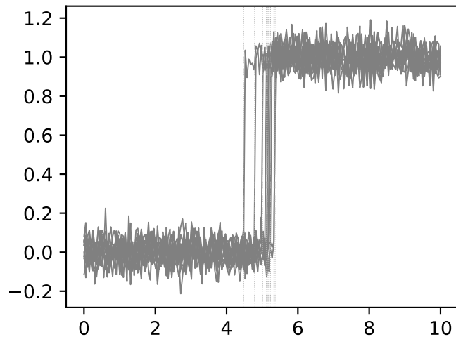
Diffuse asynchronous: unit curves
