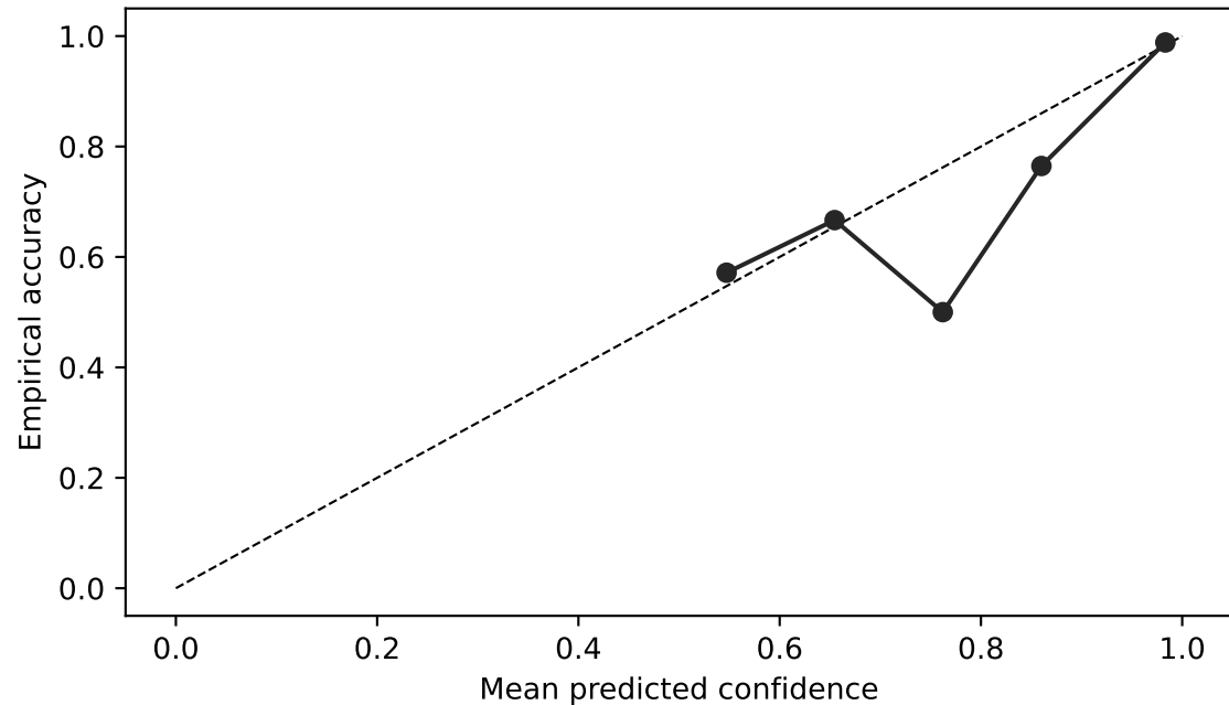
Probability calibration (locked evaluation)
