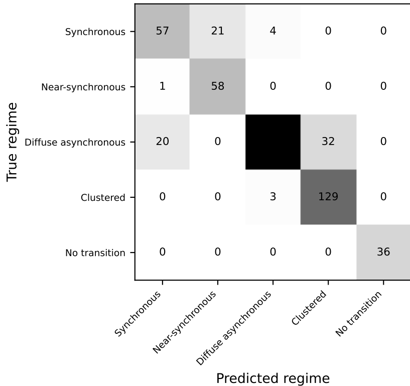
Locked-evaluation confusion matrix
