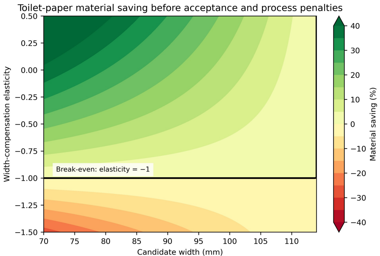
Figure 2. Toilet-paper material-saving surface as a function of candidate width and width-compensation elasticity. The black boundary marks zero saving.
