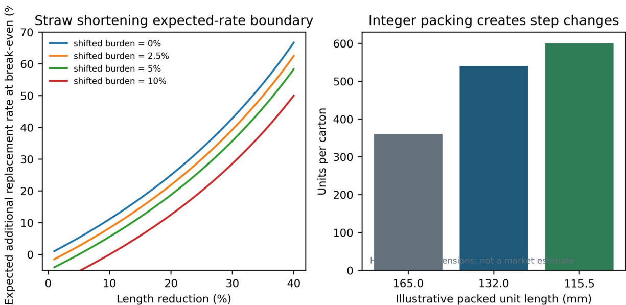
Figure 4. Straw shortening expected-additional-replacement-rate boundary and an illustrative integer-packing example. Packing dimensions are hypothetical.
