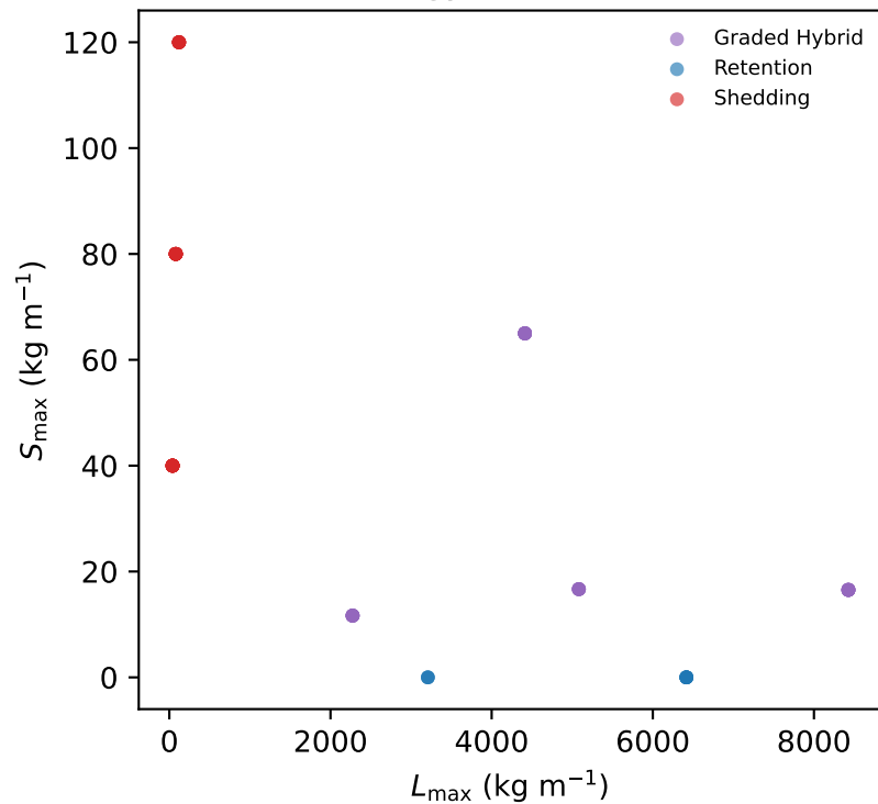
Strategy classification
