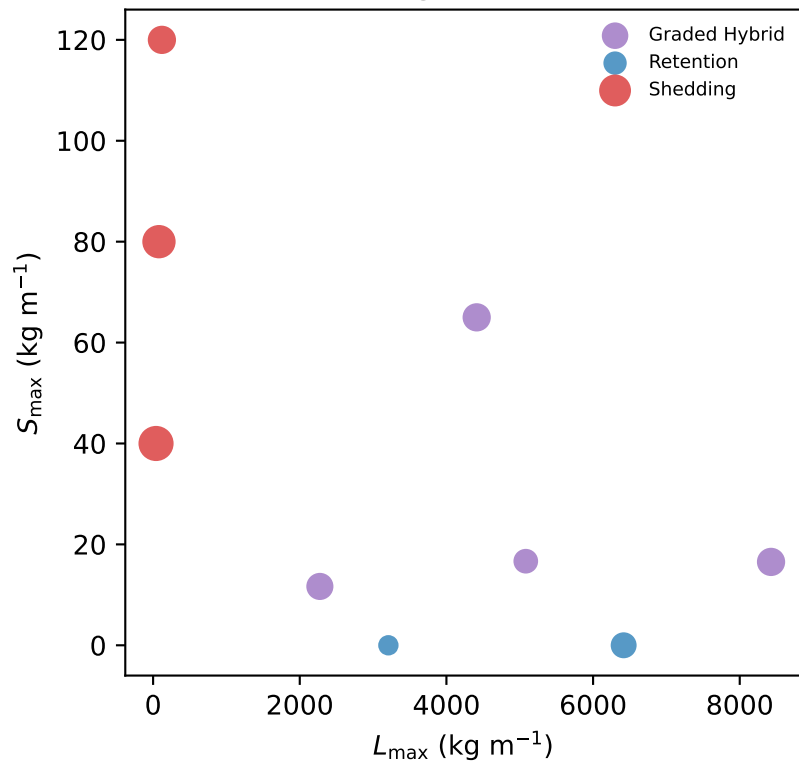
Phase-diagram selections
