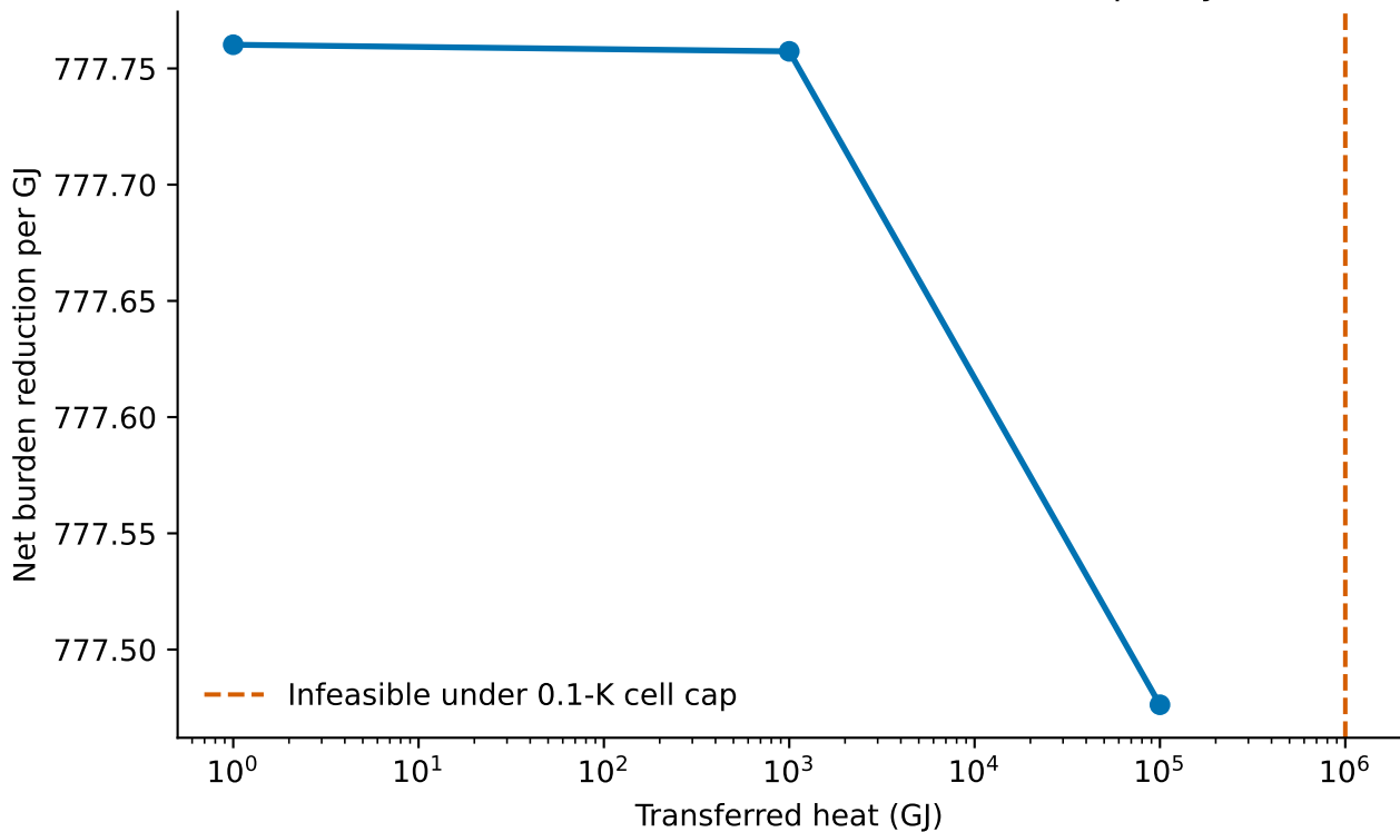
Finite-transfer results remain near-linear until capacity binds
