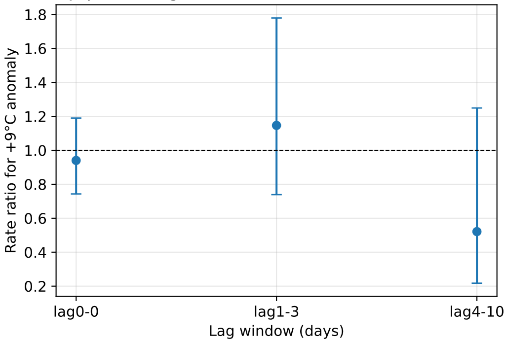
Japan C. Lag structure (wide CIs: fewer deaths)
